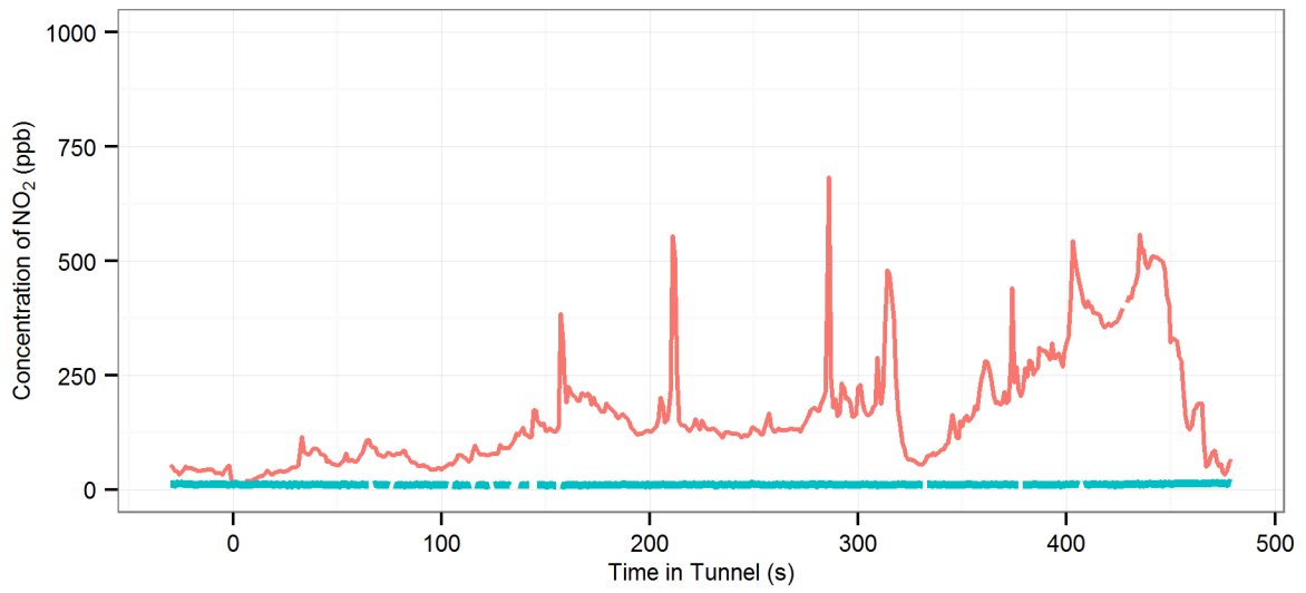
(83) MD1 (R-On | AC-On | Fn-50%) - Eastern Distributor : Southbound, 2008 Toyota Corolla
