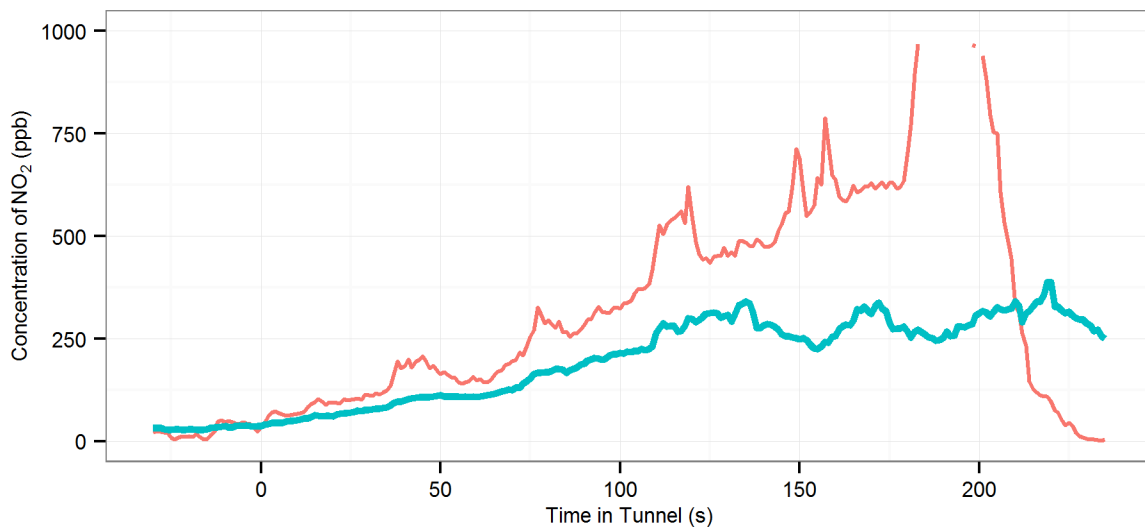
(181) MD4 (R-Off | AC-Off | Fn-50%) - Lane Cove : Eastbound, 2008 Toyota Corolla
