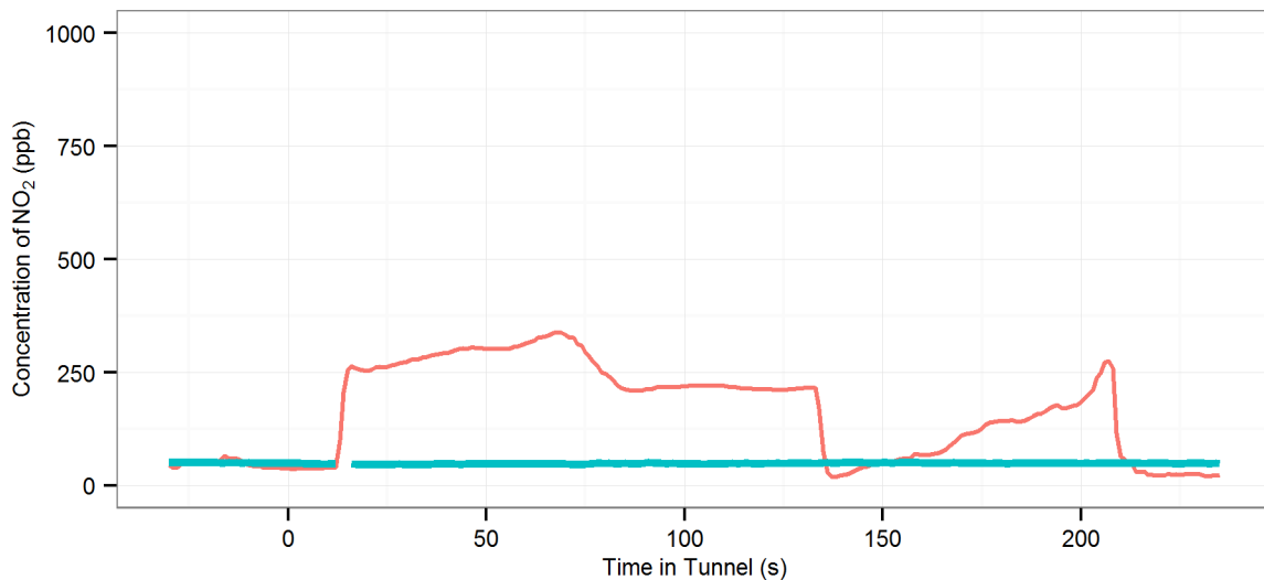
(201) MD4 (R-Off |AC-Off | Fn-50%) - M5E : Eastbound, 2002 Ford Fiesta
