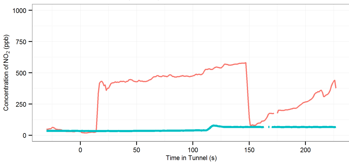
(204) MD2 (R-On | AC-Off | Fn-50%) - M5E : Eastbound, 2002 Ford Fiesta
