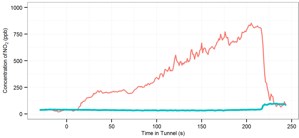
(185) MD3 (R-OnOff | AC-Off | Fn-50%) - Lane Cove : Eastbound, 2008 Toyota Corolla
