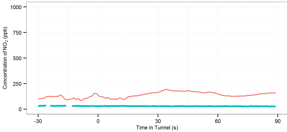
(37) MD2 (R-On | AC-Off | Fn-50%) - Eastern Distributor : Northbound, 2008 Toyota Corolla
