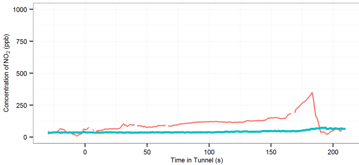
(117) MD5 (R_Off |AC-Off | Fn-0%) - Lane Cove : Westbound, 2014 Hyundai i30
