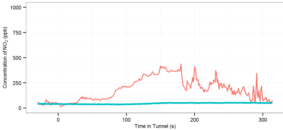
(189) MD1 (R-On | AC-On | Fn-50%) - Lane Cove : Eastbound, 2002 Fiat Punto
