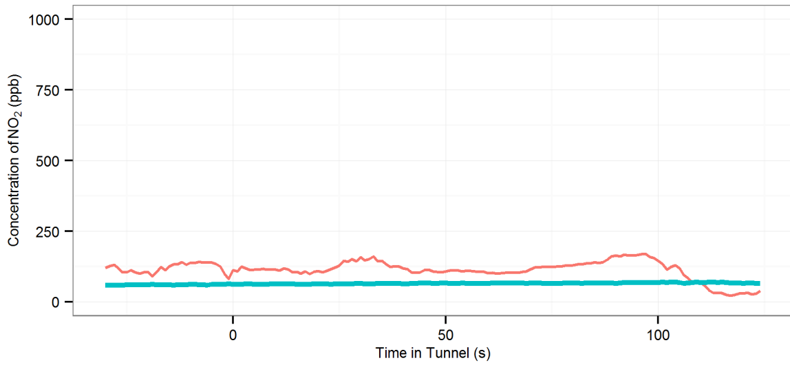
(31) MD1 (R-On | AC-On | Fn-50%) - Eastern Distributor : Northbound, 2002 Audi A3
