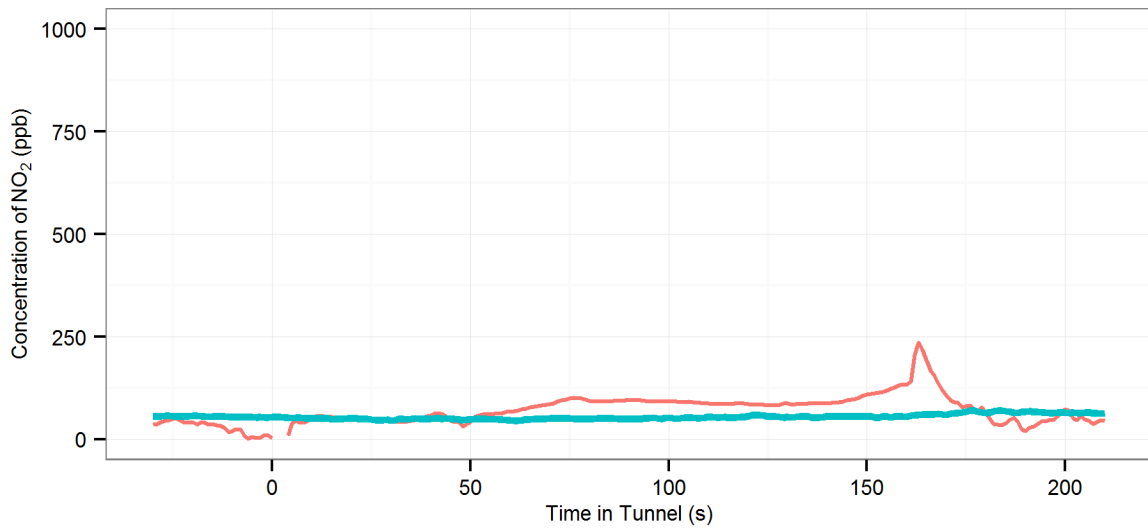
(104) MD2 (R-On | AC-Off | Fn-50%) - Lane Cove : Westbound, 2002 Ford Fiesta
