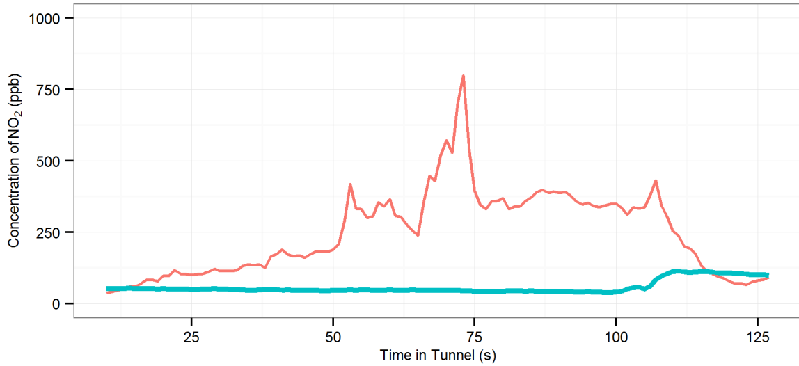
(85) MD3 (R-OnOff | AC-Off | Fn-50%) - Eastern Distributor : Southbound, 2008 Toyota Corolla
