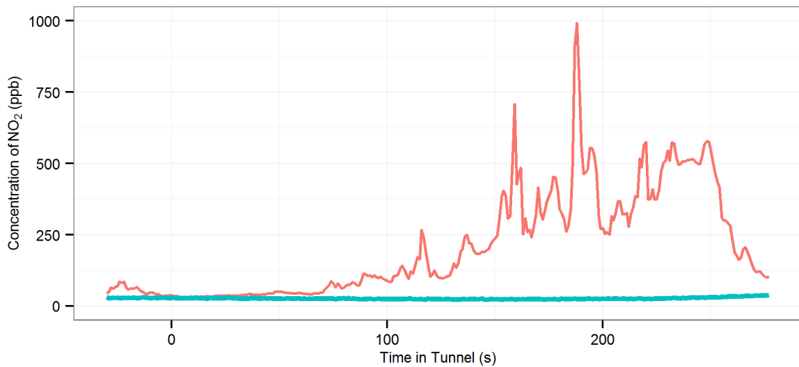
(87) MD1 (R-On | AC-On | Fn-50%) - Eastern Distributor : Southbound, 2002 Fiat Punto
