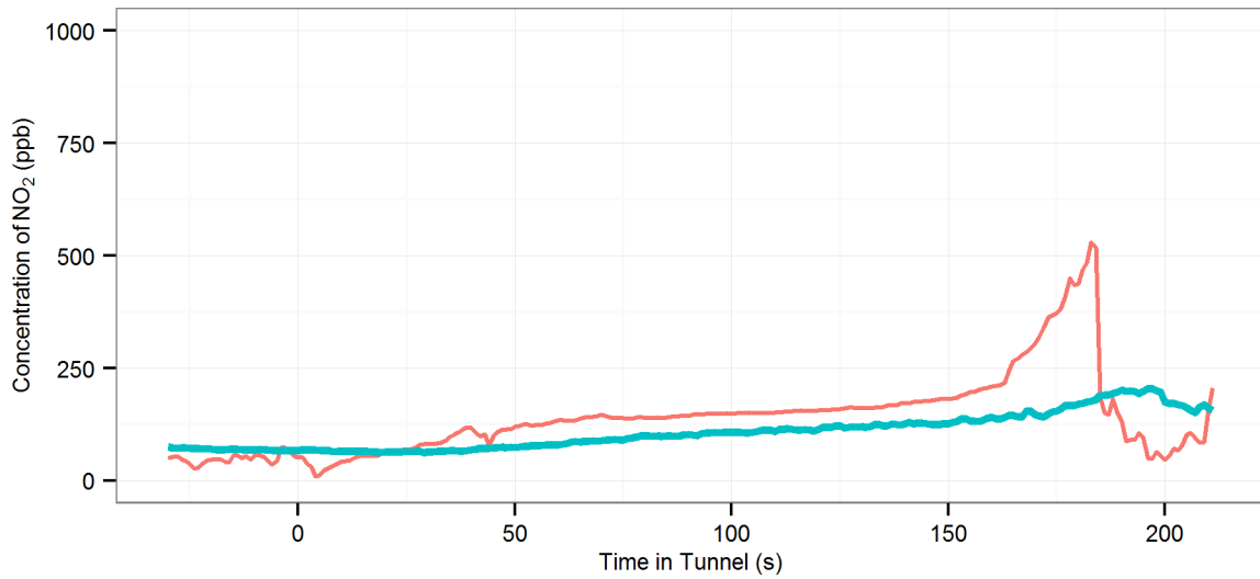
(130) MD4 (R-Off | AC-Off | Fn-50%) - Lane Cove : Westbound, 2007 Subaru Outback
