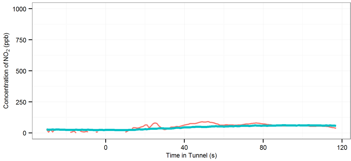
(5) MD4 (R-Off |AC-Off | Fn-50%) - Eastern Distributor : Northbound, 2008 Holden Astra Wagon
