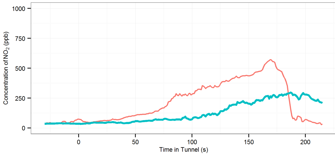
(155) MD5 (R-Off |AC-Off | Fn-0%) - Lane Cove : Eastbound, 2002 Ford Fiesta
