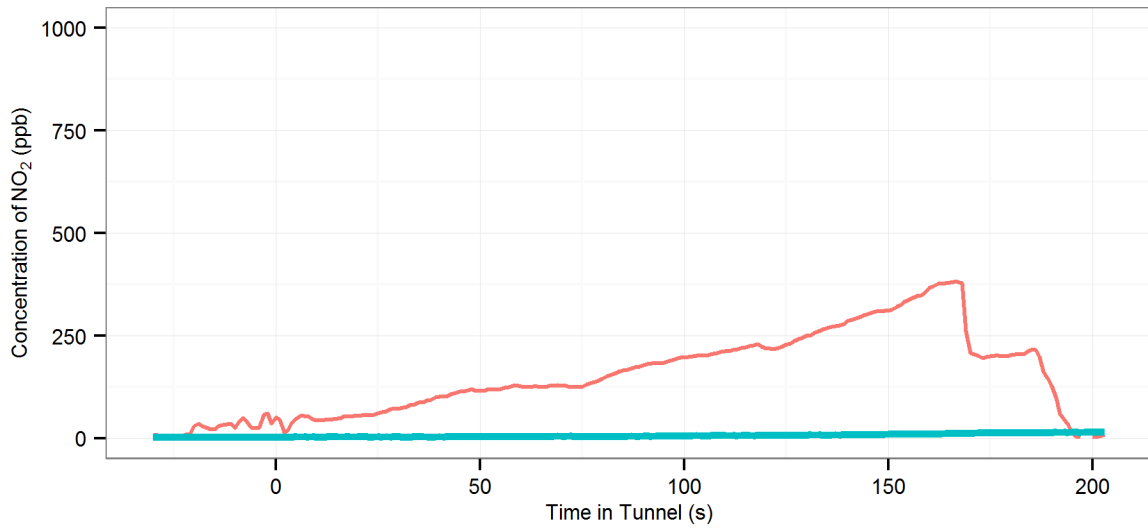
(145) MD2 (R-On | AC-Off | Fn-50%) - Lane Cove : Eastbound, 2008 Holden Astra Wagon
