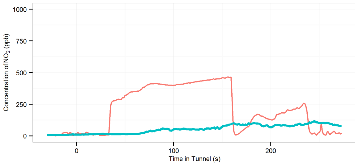
(195) MD5 (R-Off | AC-Off | Fn-0%) - M5E : Eastbound, 2008 Holden Astra Wagon
