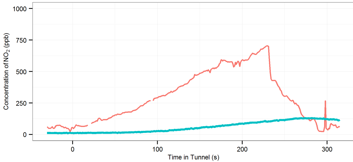
(175) MD4 (R-Off |AC-Off | Fn-50%) - Lane Cove : Eastbound, 2002 Audi A3
