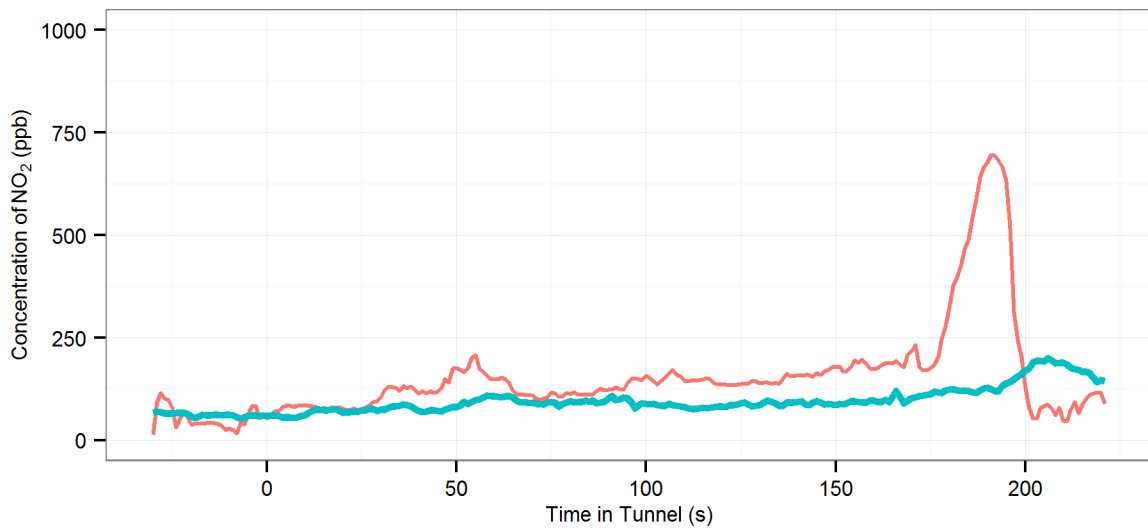
(132) MD4 (R-Off | AC-Off | Fn-50%) - Lane Cove : Westbound, 2008 Toyota Corolla
