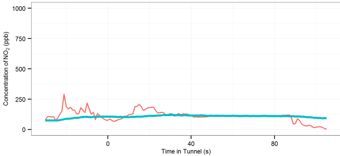
(43) MD4 (R-Off | AC-Off | Fn-50%) - Eastern Distributor : Northbound, 2002 Fiat Punto
