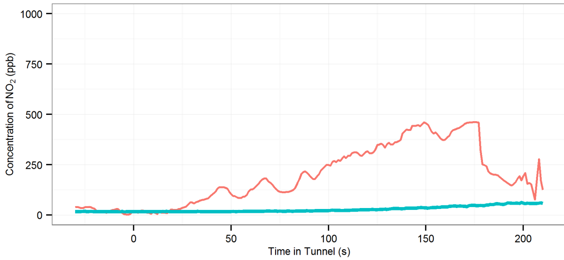
(187) MD1 (R-On | AC-On | Fn-50%) - Lane Cove : Eastbound, 2002 Fiat Punto
