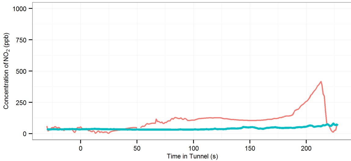
(97) MD5 (R_Off |AC-Off | Fn-0%) - Lane Cove : Westbound, 2008 Holden Astra Wagon
