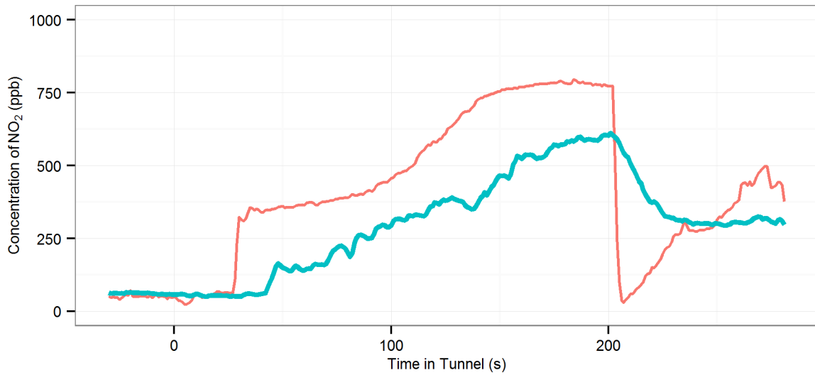
(202) MD4 (R-Off | AC-Off | Fn-50%) - M5E : Eastbound, 2002 Ford Fiesta
