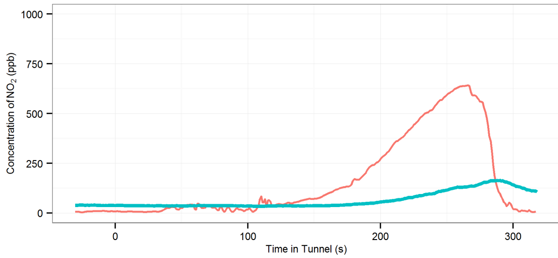
(173) MD1 (R-On | AC-On | Fn-50%) - Lane Cove : Eastbound, 2002 Audi A3
