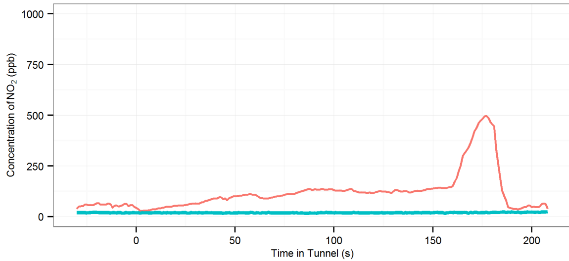
(133) MD2 (R-On | AC-Off | Fn-50%) - Lane Cove : Westbound, 2008 Toyota Corolla
