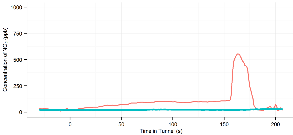
(109) MD2 (R-On | AC-Off | Fn-50%) - Lane Cove : Westbound, 2014 BMW X3
