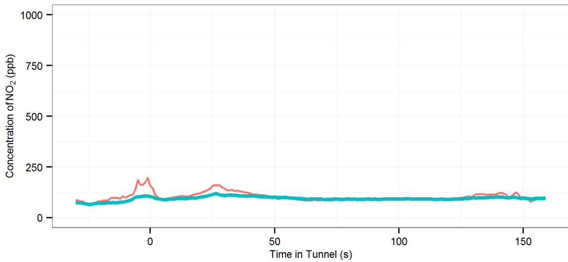
(39) MD4 (R-Off | AC-Off | Fn-50%) - Eastern Distributor : Northbound, 2008 Toyota Corolla
