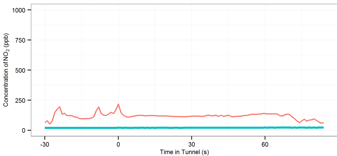
(36) MD1 (R-On | AC-On | Fn-50%) - Eastern Distributor : Northbound, 2007 Subaru Outback
