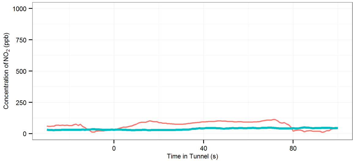
(4) MD5 (R-Off |AC-Off | Fn-0%) - Eastern Distributor : Northbound, 2008 Holden Astra Wagon
