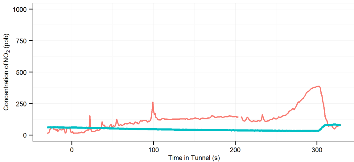
(90) MD3 (R-OnOff | AC-Off | Fn-50%) - Eastern Distributor : Southbound, 2002 Fiat Punto
