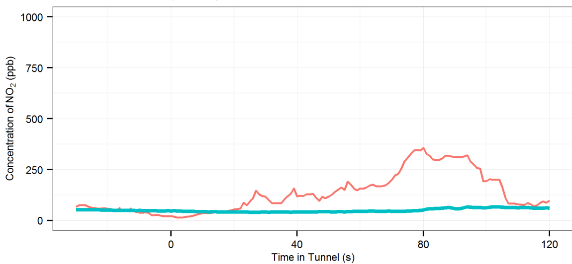
(63) MD6 (R_Off |AC-Off | Fn-100%) - Eastern Distributor : Southbound, 2014 BMW X3
