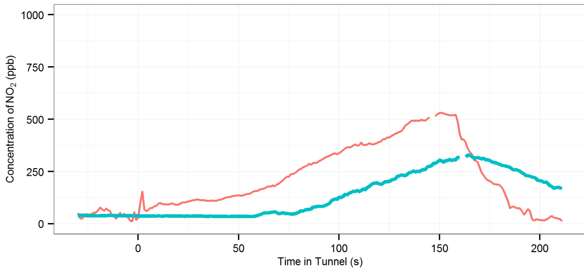
(179) MD1 (R-On | AC-On | Fn-50%) - Lane Cove : Eastbound, 2007 Subaru Outback
