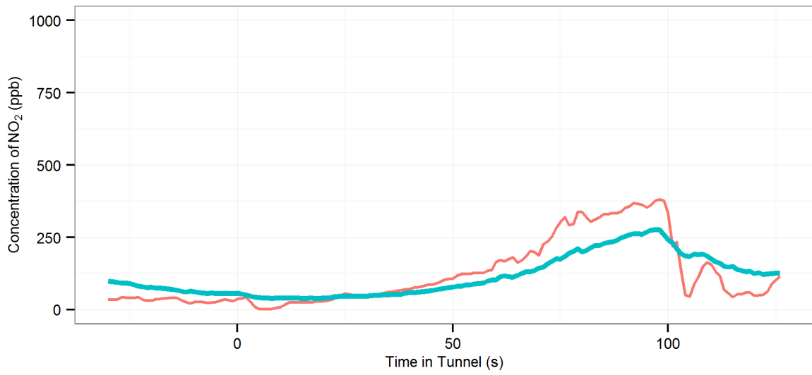
(50) MD6 (R_Off |AC-Off | Fn-100%) - Eastern Distributor : Southbound, 2008 Holden Astra Wagon
