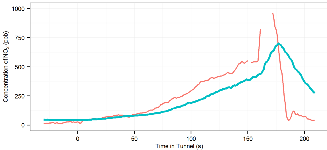
(153) MD6 (R_Off |AC-Off | Fn-100%) - Lane Cove : Eastbound, 2002 Ford Fiesta
