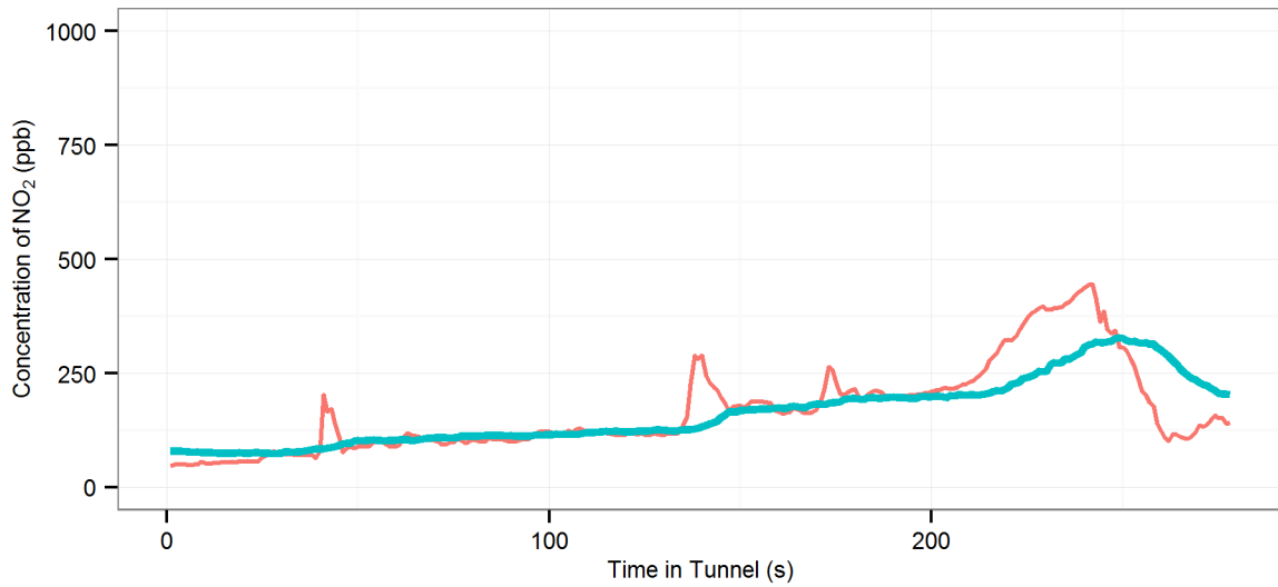
(55) MD6 (R_Off |AC-Off | Fn-100%) - Eastern Distributor : Southbound, 2002 Ford Fiesta
