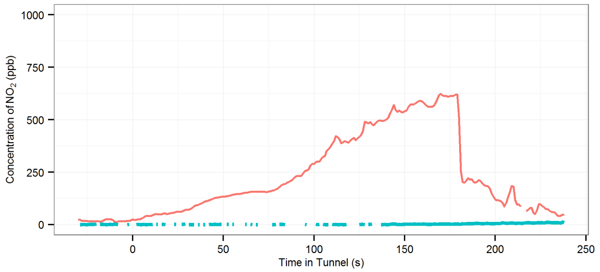
(158) MD5 (R-Off |AC-Off | Fn-0%) - Lane Cove : Eastbound, 2014 BMW X3
