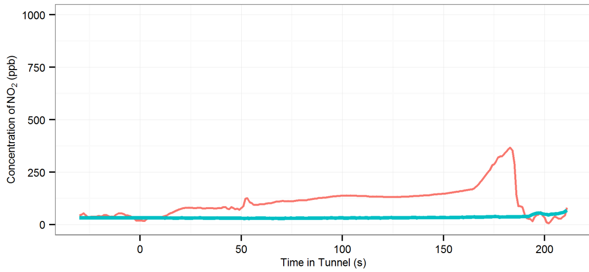
(140) MD2 (R-On | AC-Off | Fn-50%) - Lane Cove : Westbound, 2002 Fiat Punto
