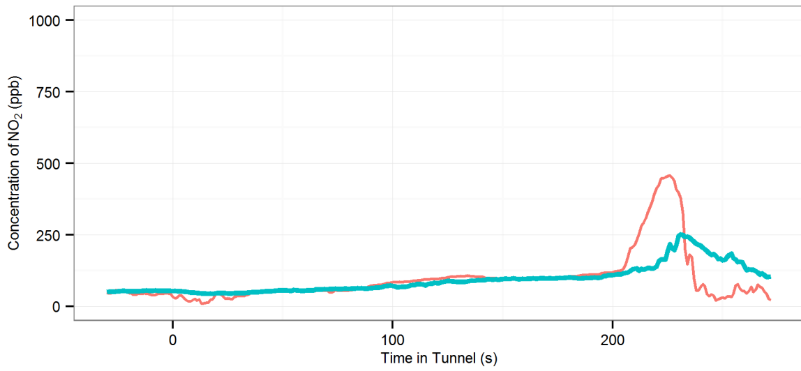
(98) MD6 (R_Off |AC-Off | Fn-100%) - Lane Cove : Westbound, 2008 Holden Astra Wagon
