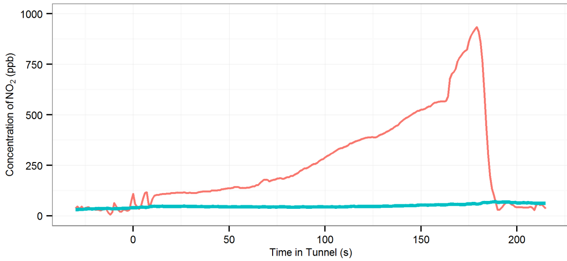
(178) MD2 (R-On | AC-Off | Fn-50%) - Lane Cove : Eastbound, 2007 Subaru Outback
