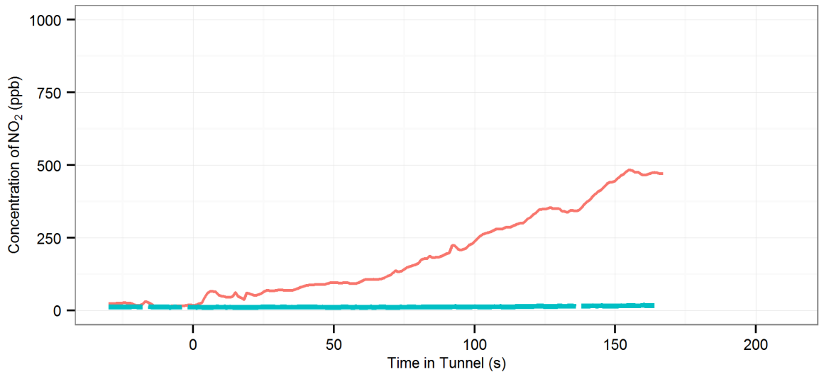
(184) MD1 (R-On | AC-On | Fn-50%) - Lane Cove : Eastbound, 2008 Toyota Corolla
