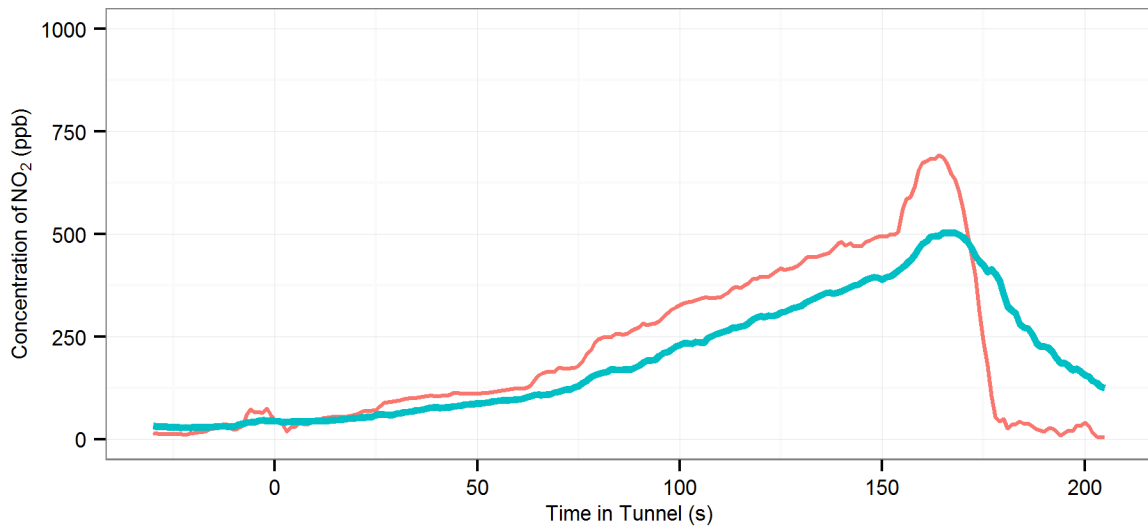
(161) MD6 (R_Off | AC-Off | Fn-100%) - Lane Cove : Eastbound, 2014 Hyundai i30
