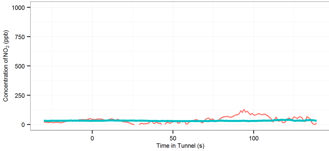
(2) MD5 (R-Off | AC-Off | Fn-0%) - Eastern Distributor : Northbound, 2008 Holden Astra Wagon
