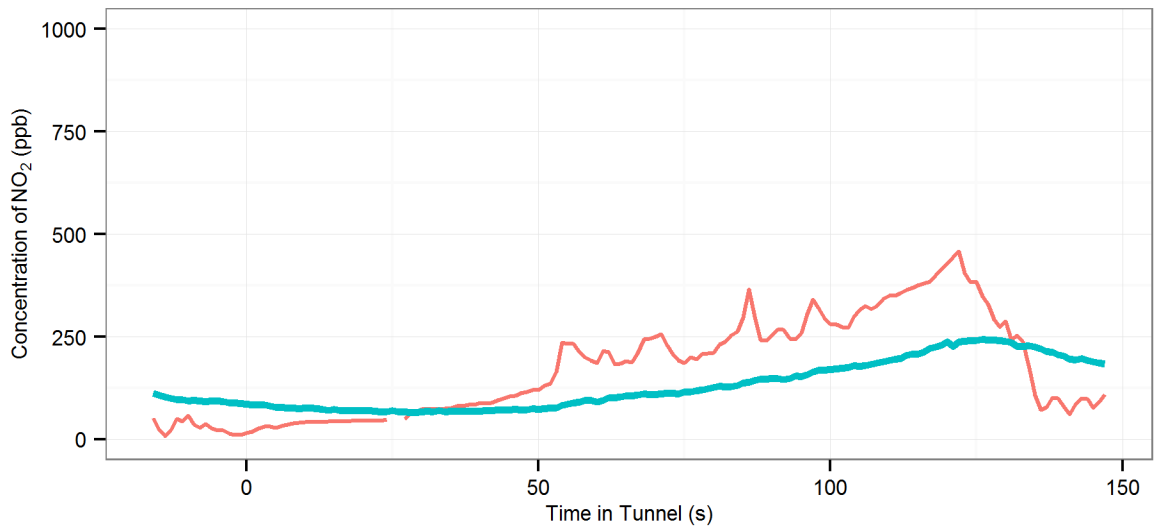
(68) MD4 (R-Off | AC-Off | Fn-50%) - Eastern Distributor : Southbound, 2014 Hyundai i30
