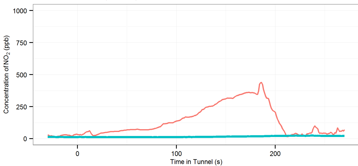
(147) MD2 (R-On | AC-Off | Fn-50%) - Lane Cove : Eastbound, 2008 Holden Astra Wagon
