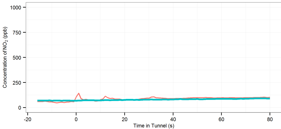
(45) MD4 (R-Off | AC-Off | Fn-50%) - Eastern Distributor : Northbound, 2002 Fiat Punto
