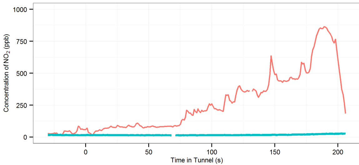
(180) MD1 (R-On | AC-On | Fn-50%) - Lane Cove : Eastbound, 2008 Toyota Corolla
