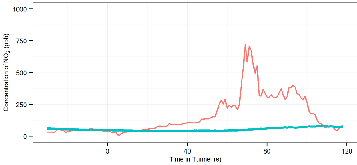
(77) MD3 (R-OnOff | AC-Off | Fn-50%) - Eastern Distributor : Southbound, 2002 Audi A3
