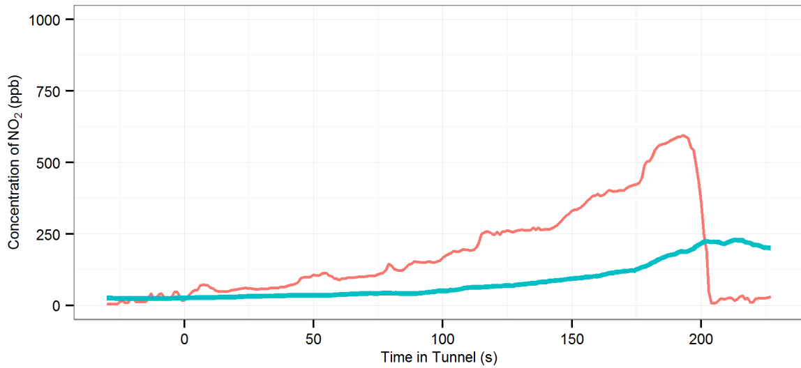
(151) MD5 (R-Off |AC-Off | Fn-0%) - Lane Cove : Eastbound, 2002 Ford Fiesta
