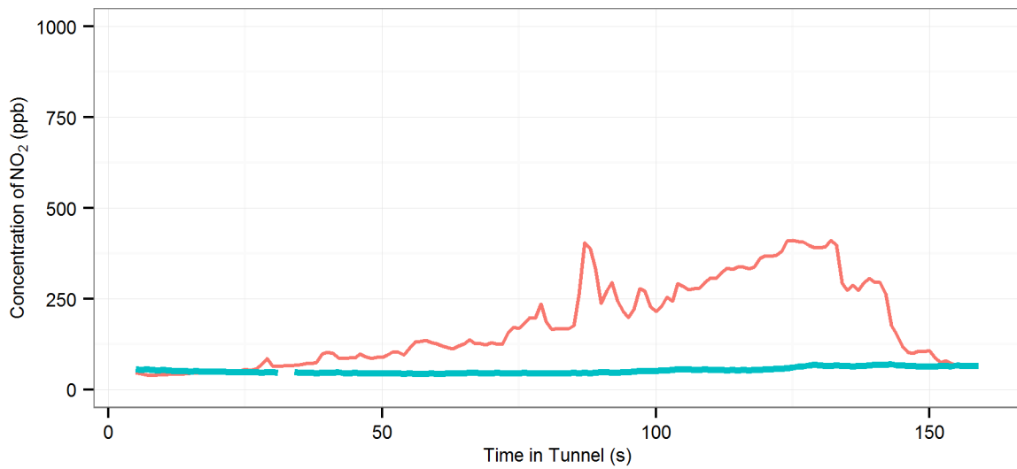
(72) MD2 (R-On | AC-Off | Fn-50%) - Eastern Distributor : Southbound, 2002 Audi A3
