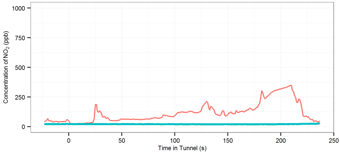
(91) MD1 (R-On | AC-On | Fn-50%) - Eastern Distributor : Southbound, 2002 Fiat Punto
