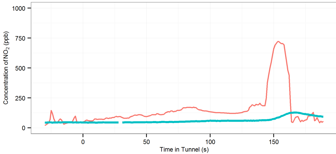
(121) MD1 (R-On | AC-On | Fn-50%) - Lane Cove : Westbound, 2002 Audi A3
