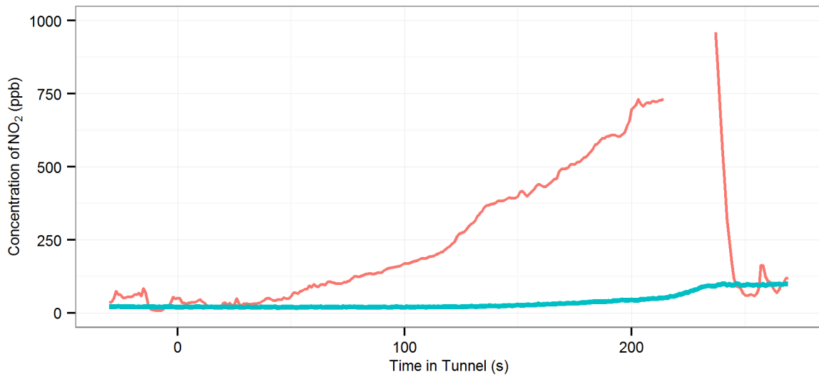
(188) MD1 (R-On | AC-On | Fn-50%) - Lane Cove : Eastbound, 2002 Fiat Punto
