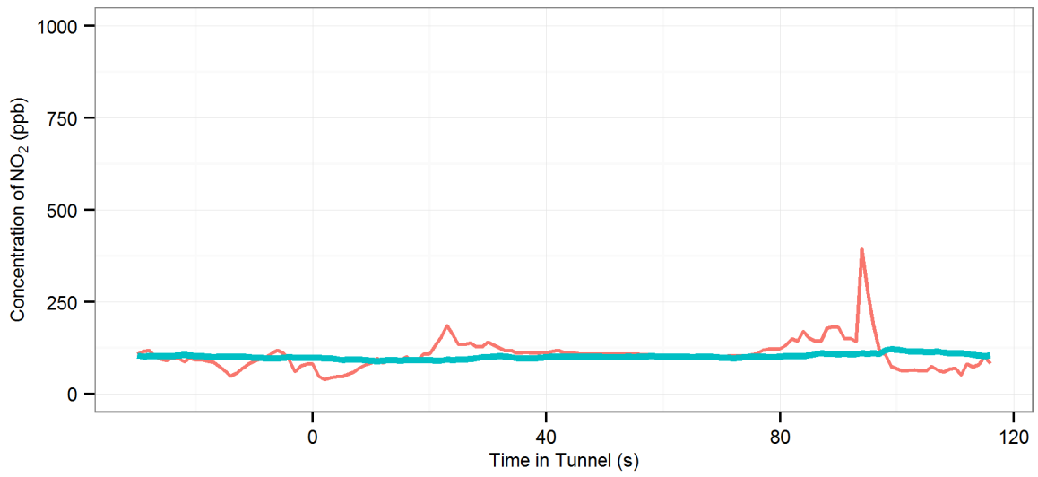
(35) MD4 (R-Off | AC-Off | Fn-50%) - Eastern Distributor : Northbound, 2007 Subaru Outback
