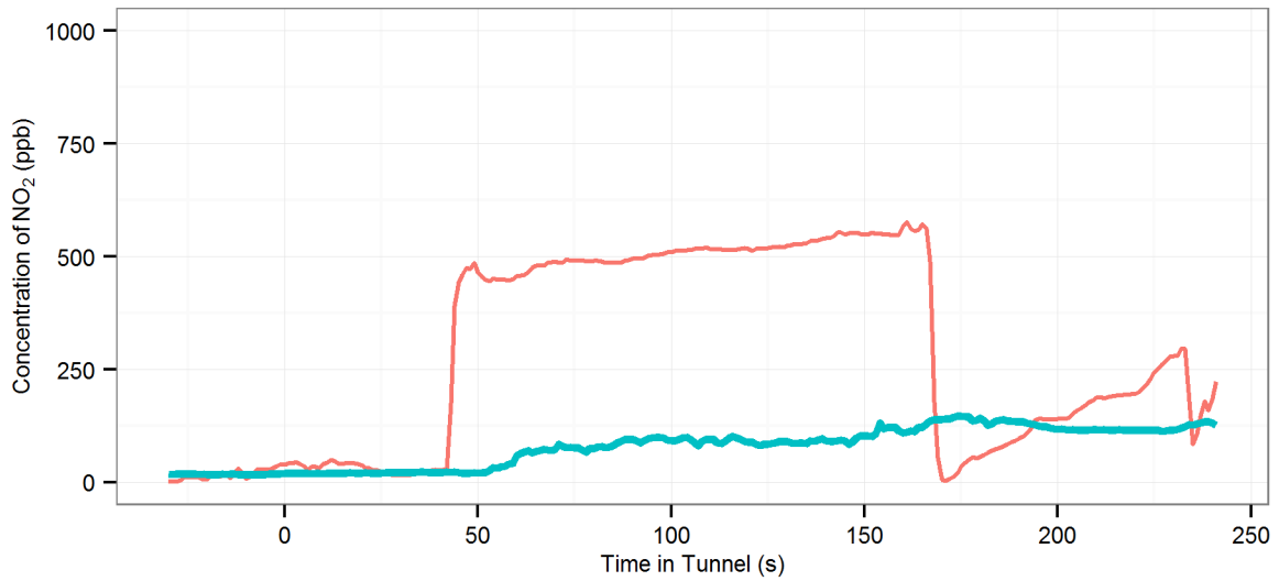
(196) MD5 (R-Off |AC-Off | Fn-0%) - M5E : Eastbound, 2008 Holden Astra Wagon
