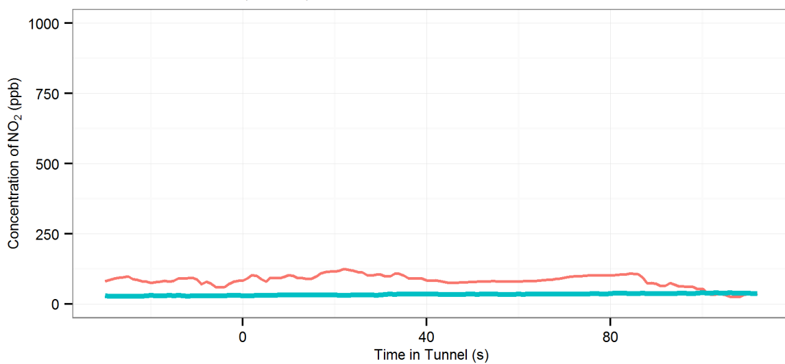
(27) MD4 (R-Off | AC-Off | Fn-50%) - Eastern Distributor : Northbound, 2002 Audi A3
