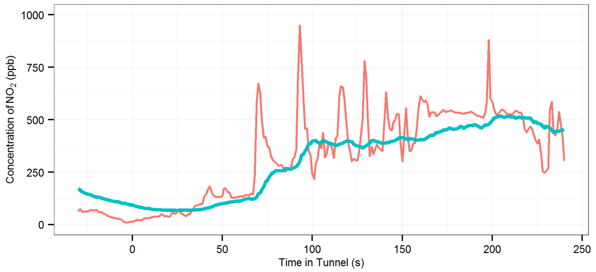
(59) MD6 (R_Off |AC-Off | Fn-100%) - Eastern Distributor : Southbound, 2002 Ford Fiesta
