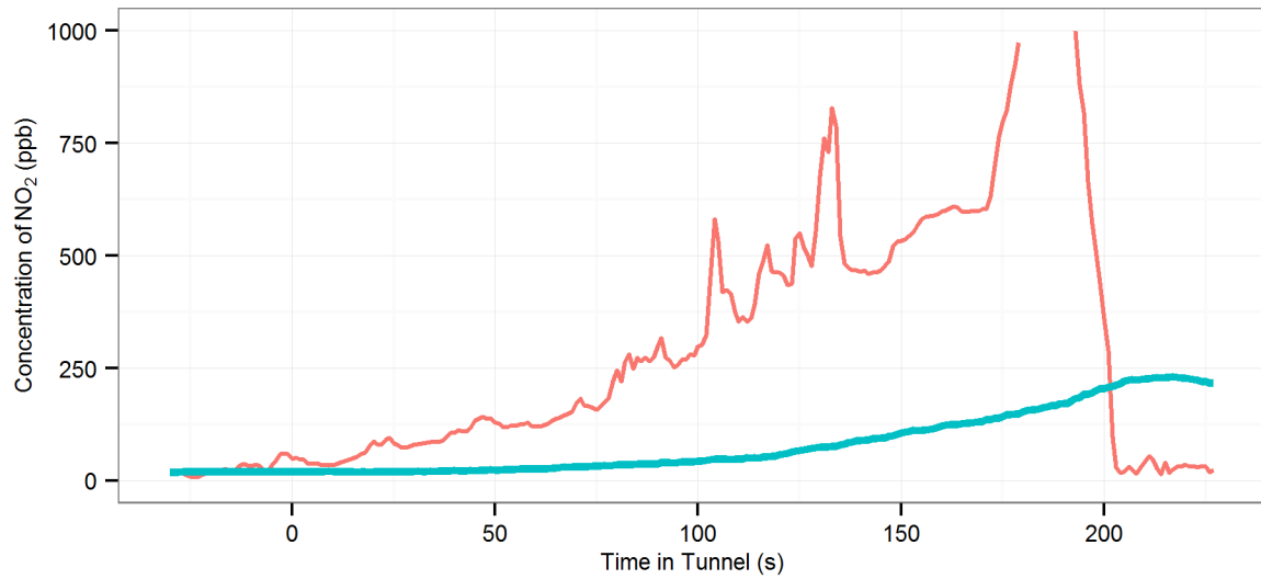
(172) MD2 (R-On | AC-Off | Fn-50%) - Lane Cove : Eastbound, 2002 Audi A3
