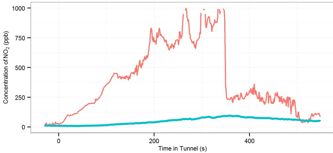
(169) MD1 (R-On | AC-On | Fn-50%) - Lane Cove : Eastbound, 2002 Audi A3
