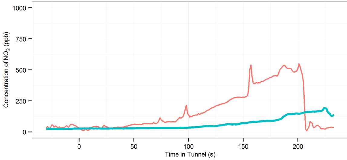
(152) MD5 (R-Off |AC-Off | Fn-0%) - Lane Cove : Eastbound, 2002 Ford Fiesta
