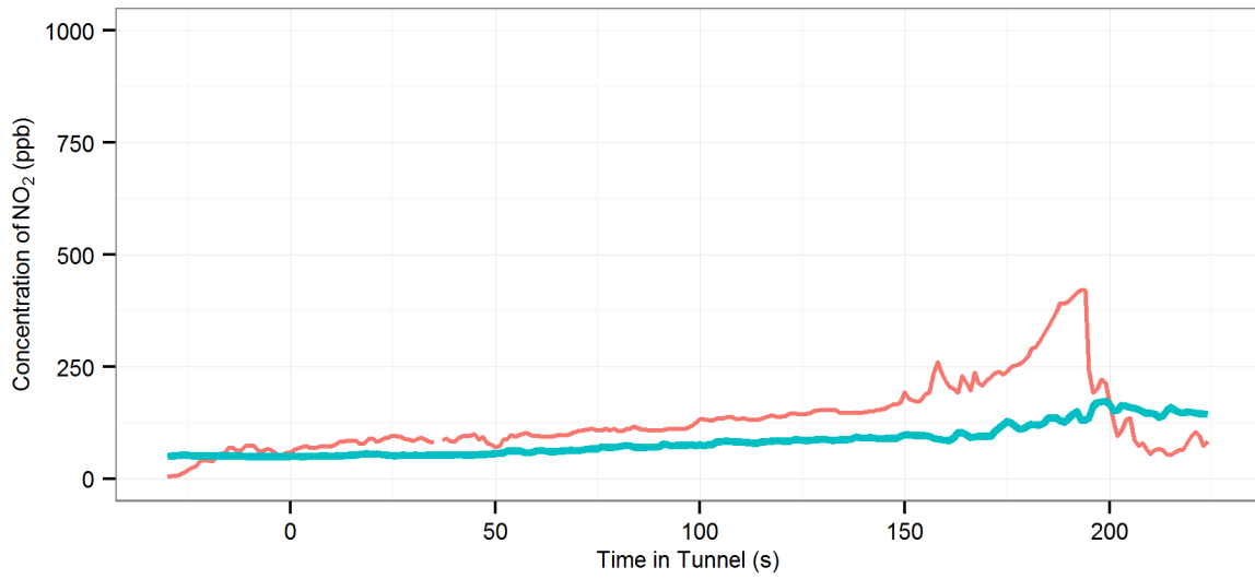
(100) MD5 (R-Off |AC-Off | Fn-0%) - Lane Cove : Westbound, 2002 Ford Fiesta
