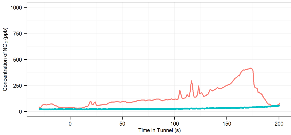
(74) MD4 (R-Off | AC-Off | Fn-50%) - Eastern Distributor : Southbound, 2002 Audi A3
