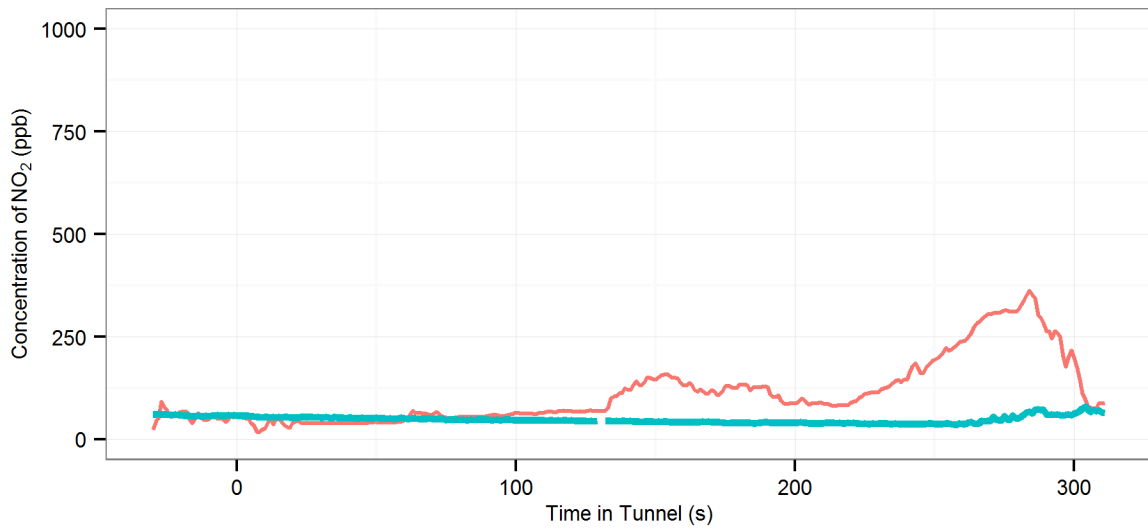
(56) MD5 (R-Off |AC-Off | Fn-0%) - Eastern Distributor : Southbound, 2002 Ford Fiesta
