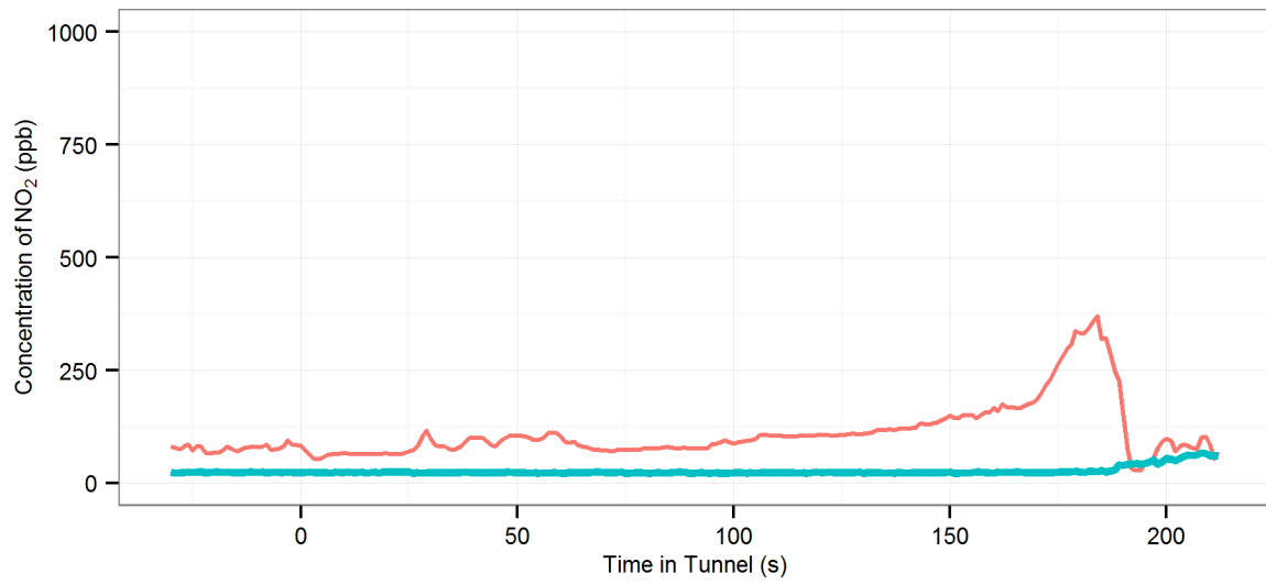
(137) MD2 (R-On | AC-Off | Fn-50%) - Lane Cove : Westbound, 2002 Fiat Punto
