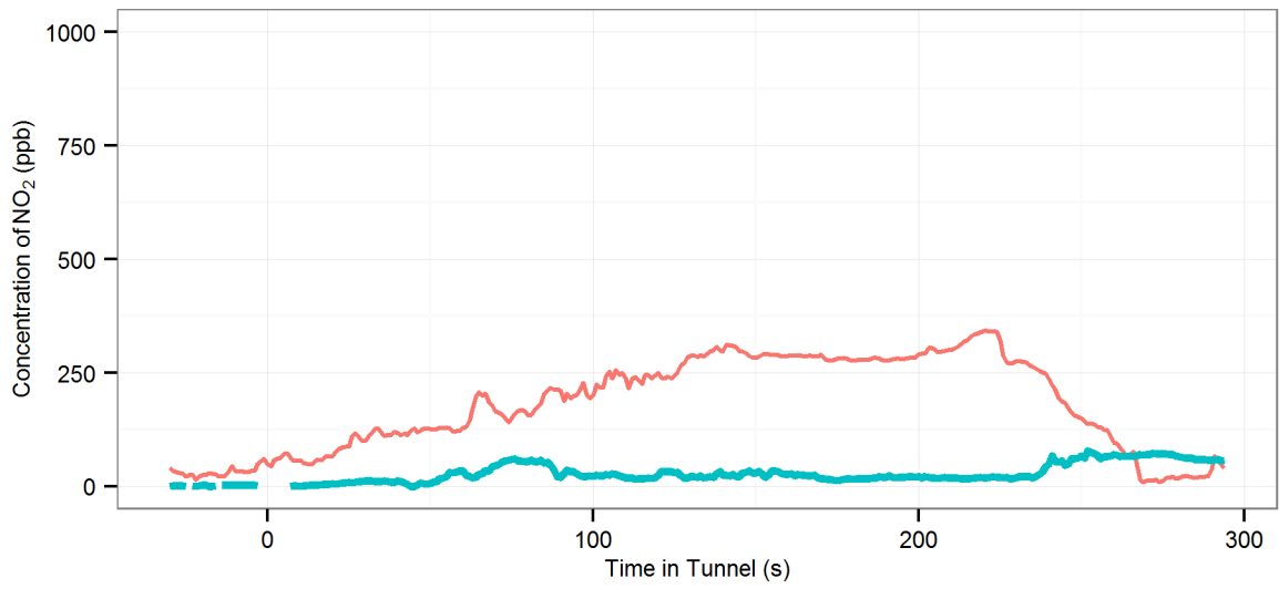
(143) MD5 (R-Off | AC-Off | Fn-0%) - Lane Cove : Eastbound, 2008 Holden Astra Wagon
