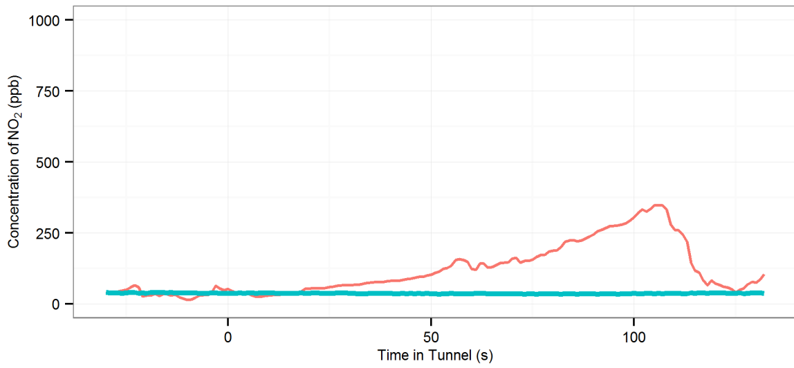
(89) MD1 (R-On | AC-On | Fn-50%) - Eastern Distributor : Southbound, 2002 Fiat Punto
