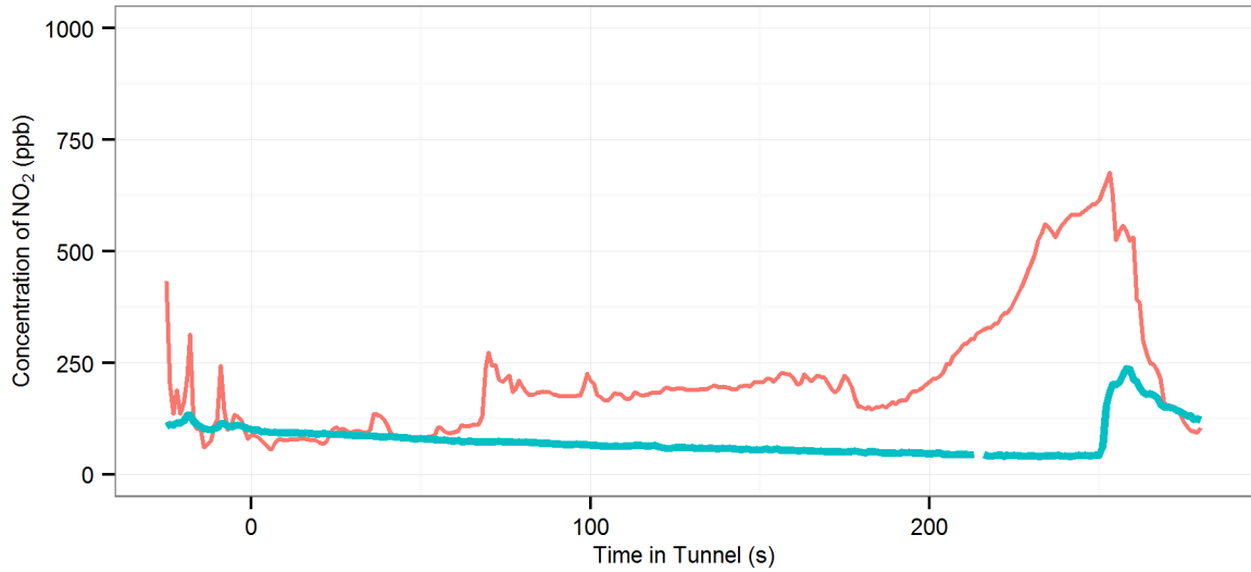
(82) MD3 (R-OnOff | AC-Off | Fn-50%) - Eastern Distributor : Southbound, 2008 Toyota Corolla
