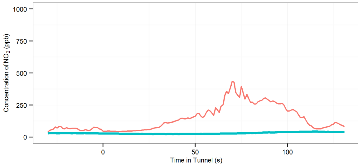
(71) MD1 (R-On | AC-On | Fn-50%) - Eastern Distributor : Southbound, 2002 Audi A3
