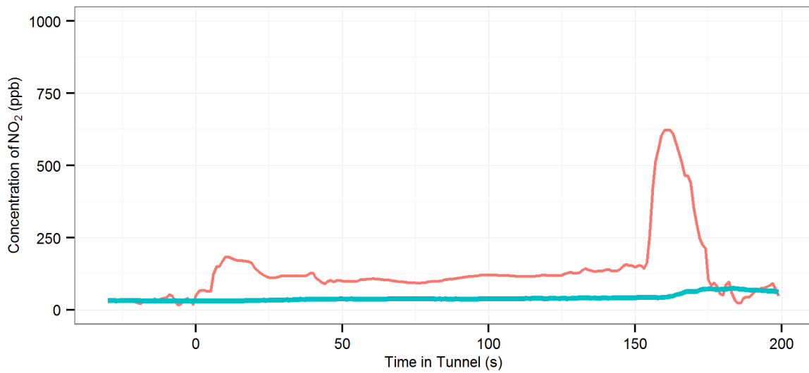
(120) MD3 (R-OnOff | AC-Off | Fn-50%) - Lane Cove : Westbound, 2002 Audi A3
