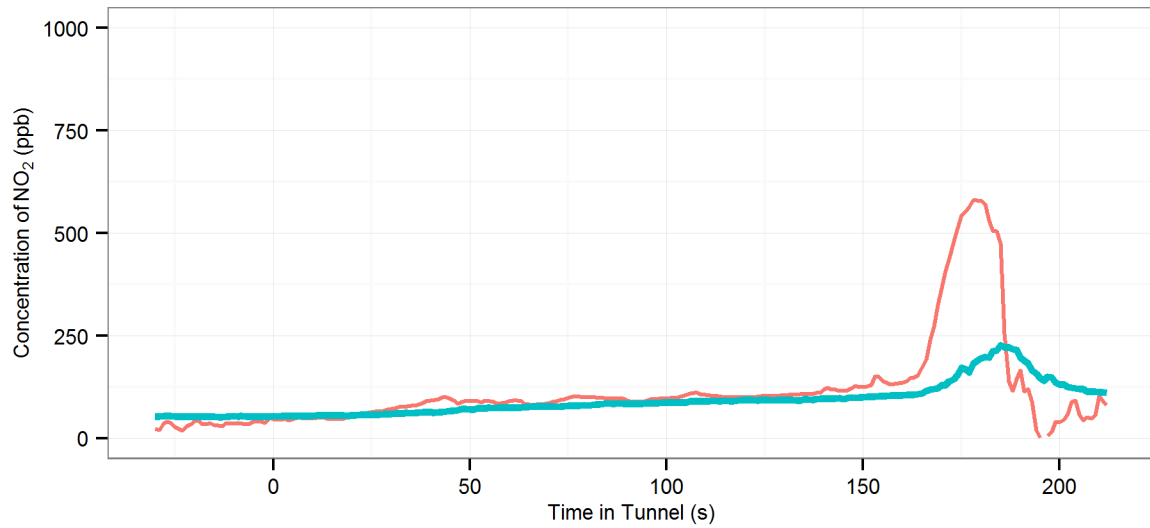
(139) MD4 (R-Off | AC-Off | Fn-50%) - Lane Cove : Westbound, 2002 Fiat Punto
