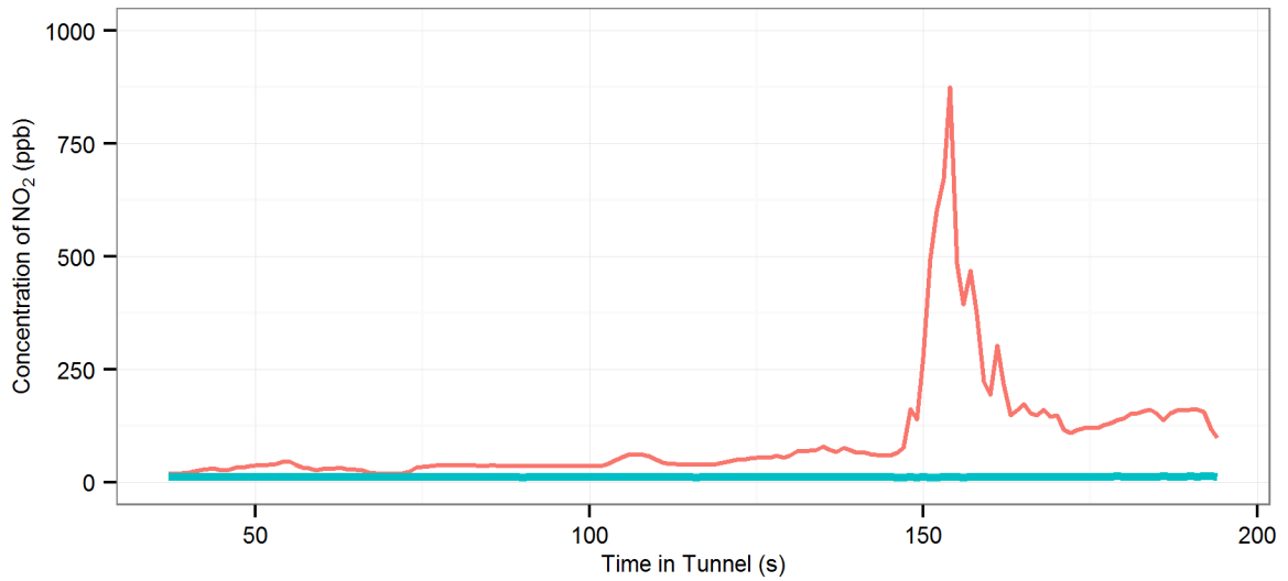
(52) MD2 (R-On | AC-Off | Fn-50%) - Eastern Distributor : Southbound, 2008 Holden Astra Wagon
