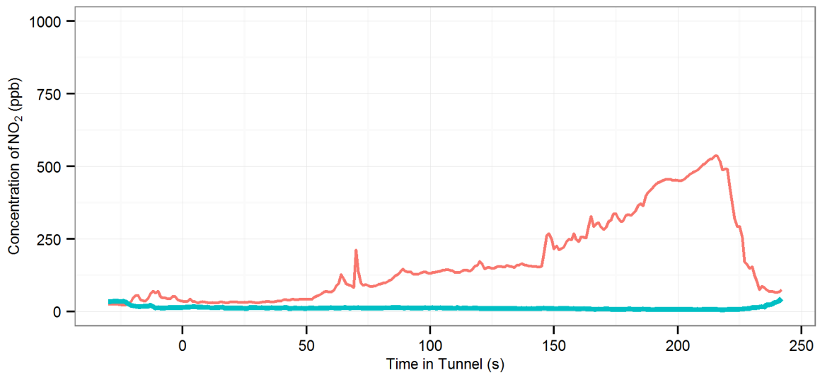
(54) MD5 (R-Off | AC-Off | Fn-0%) - Eastern Distributor : Southbound, 2008 Holden Astra Wagon
