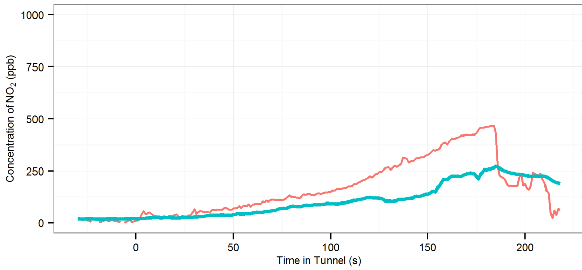
(146) MD4 (R-Off | AC-Off | Fn-50%) - Lane Cove : Eastbound, 2008 Holden Astra Wagon
