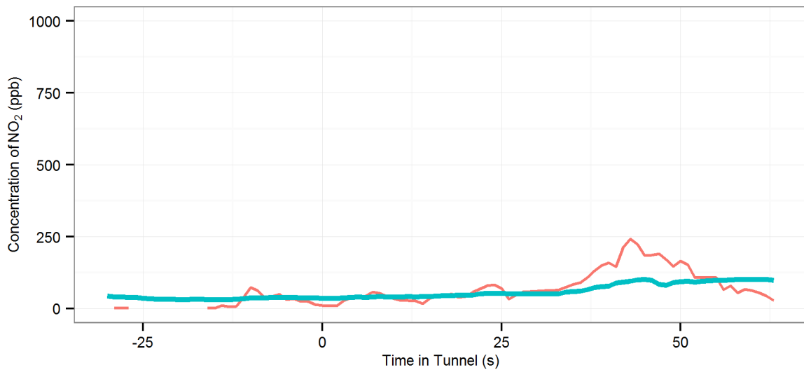
(3) MD6 (R_Off | AC-Off | Fn-100%) - Eastern Distributor : Northbound, 2008 Holden Astra Wagon
