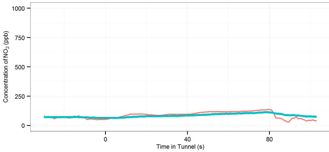
(23) MD6 (R_Off |AC-Off | Fn-100%) - Eastern Distributor : Northbound, 2014 Hydunai i30
