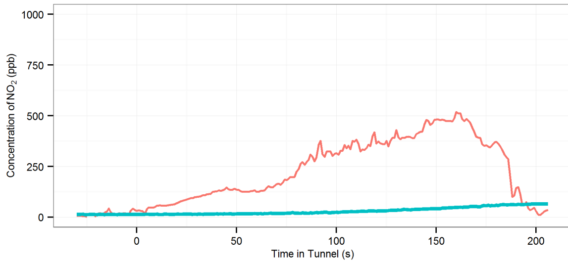
(191) MD1 (R-On | AC-On | Fn-50%) - Lane Cove : Eastbound, 2002 Fiat Punto
