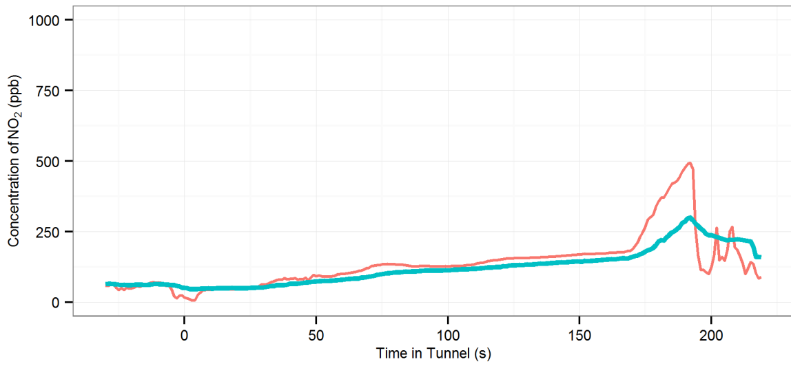
(113) MD6 (R_Off | AC-Off | Fn-100%) - Lane Cove : Westbound, 2014 Hyundai i30
