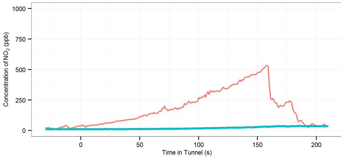
(176) MD3 (R-OnOff |AC-Off | Fn-50%) - Lane Cove : Eastbound, 2007 Subaru Outback
