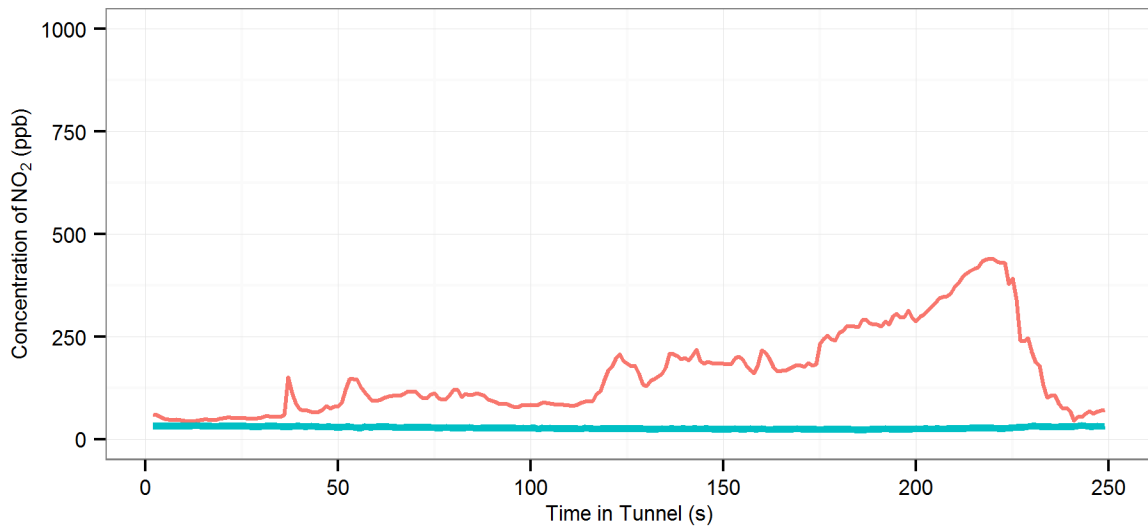
(86) MD1 (R-On | AC-On | Fn-50%) - Eastern Distributor : Southbound, 2002 Fiat Punto
