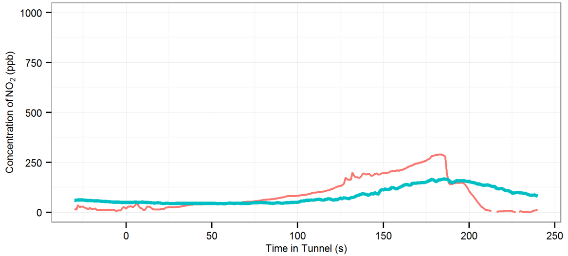
(148) MD5 (R-Off |AC-Off | Fn-0%) - Lane Cove : Eastbound, 2008 Holden Astra Wagon
