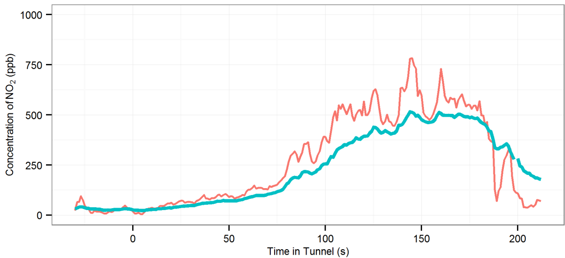
(144) MD6 (R_Off | AC-Off | Fn-100%) - Lane Cove : Eastbound, 2008 Holden Astra Wagon
