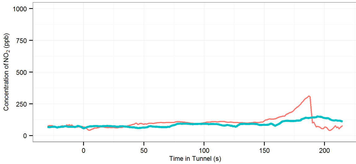
(103) MD4 (R-Off | AC-Off | Fn-50%) - Lane Cove : Westbound, 2002 Ford Fiesta
