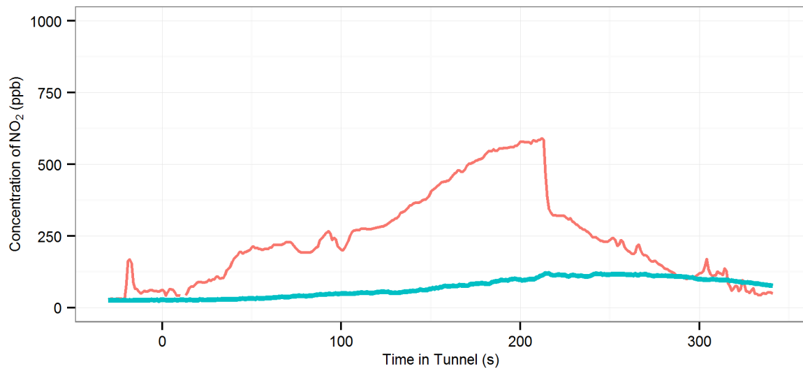
(168) MD2 (R-On | AC-Off | Fn-50%) - Lane Cove : Eastbound, 2002 Audi A3
