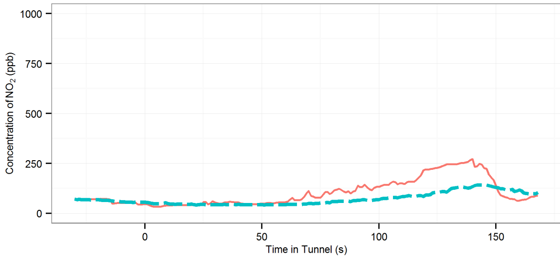
(61) MD6 (R_Off |AC-Off | Fn-100%) - Eastern Distributor : Southbound, 2014 BMW X3
