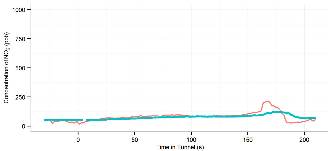
(138) MD4 (R-Off | AC-Off | Fn-50%) - Lane Cove : Westbound, 2002 Fiat Punto
