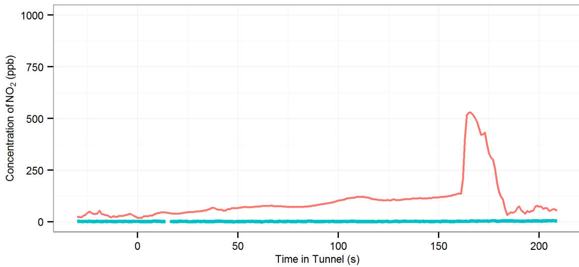
(114) MD2 (R-On | AC-Off | Fn-50%) - Lane Cove : Westbound, 2014 Hyundai i30
