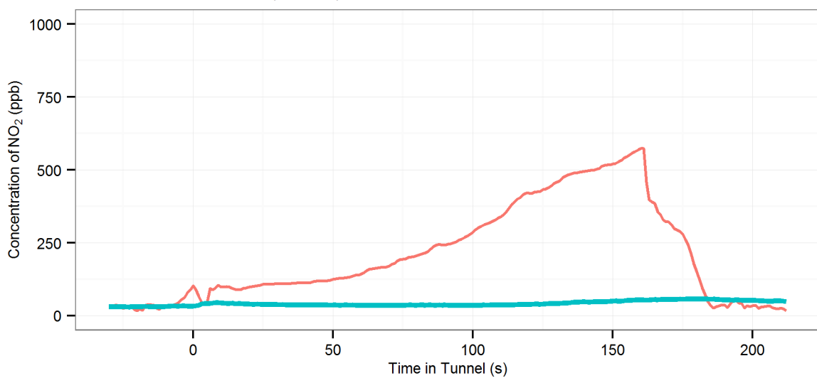
(177) MD3 (R-OnOff |AC-Off | Fn-50%) - Lane Cove : Eastbound, 2007 Subaru Outback
