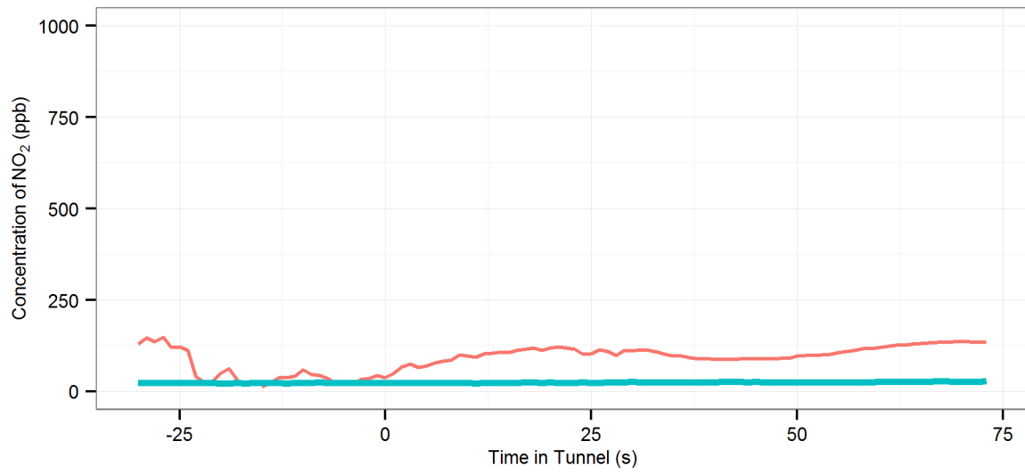
(47) MD2 (R-On | AC-Off | Fn-50%) - Eastern Distributor : Northbound, 2002 Fiat Punto
