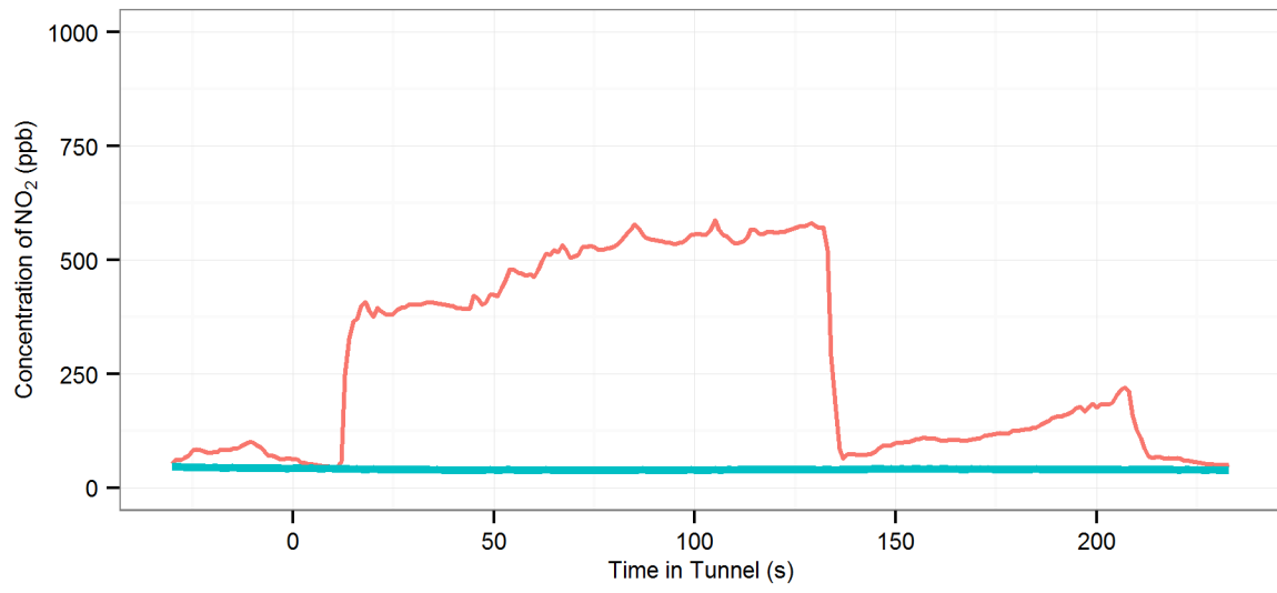
(208) MD2 (R-On | AC-Off | Fn-50%) - M5E : Eastbound, 2014 BMW X3
