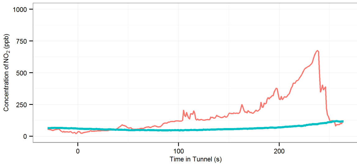
(75) MD2 (R-On | AC-Off | Fn-50%) - Eastern Distributor : Southbound, 2002 Audi A3
