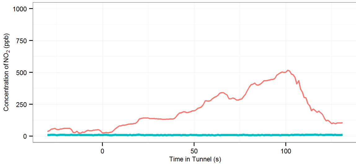
(64) MD2 (R-On | AC-Off | Fn-50%) - Eastern Distributor : Southbound, 2014 Hyundai i30
