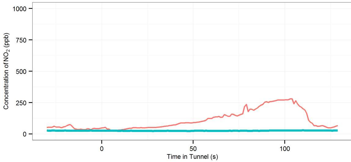
(79) MD3 (R-OnOff | AC-Off | Fn-50%) - Eastern Distributor : Southbound, 2007 Subaru Outback
