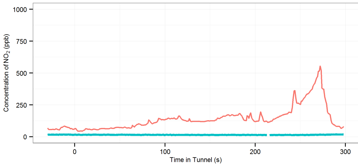
(84) MD1 (R-On | AC-On | Fn-50%) - Eastern Distributor : Southbound, 2008 Toyota Corolla
