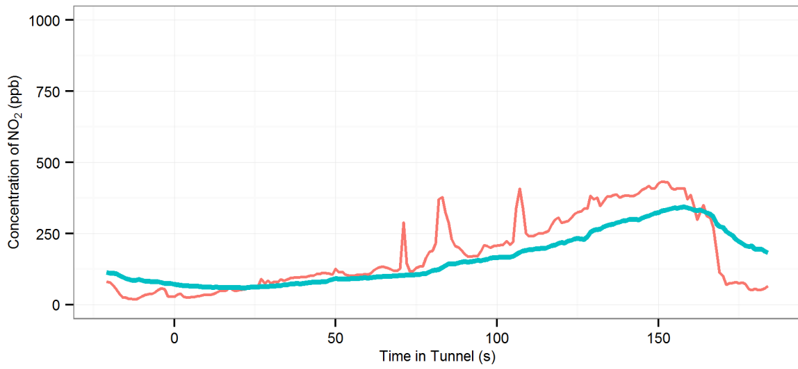
(65) MD6 (R_Off | AC-Off | Fn-100%) - Eastern Distributor : Southbound, 2014 Hyundai i30
