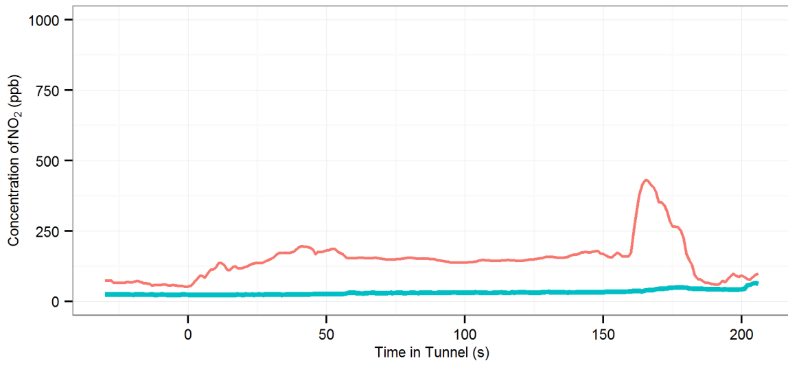
(107) MD4 (R-Off | AC-Off | Fn-50%) - Lane Cove : Westbound, 2014 BMW X3
