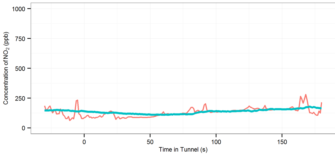
(9) MD4 (R-Off | AC-Off | Fn-50%) - Eastern Distributor : Northbound, 2002 Ford Fiesta
