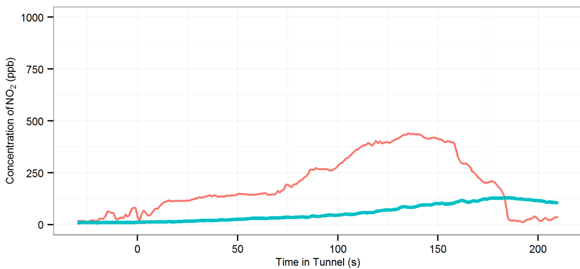
(171) MD1 (R-On | AC-On | Fn-50%) - Lane Cove : Eastbound, 2002 Audi A3
