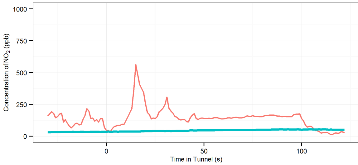
(32) MD2 (R-On | AC-Off | Fn-50%) - Eastern Distributor : Northbound, 2002 Audi A3
