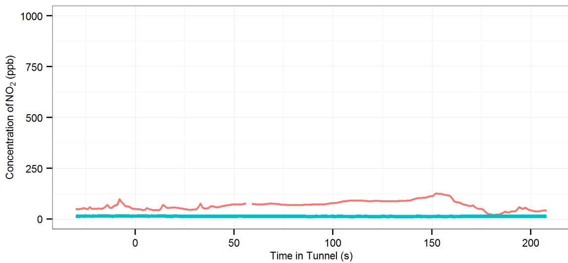
(108) MD2 (R-On | AC-Off | Fn-50%) - Lane Cove : Westbound, 2014 BMW X3
