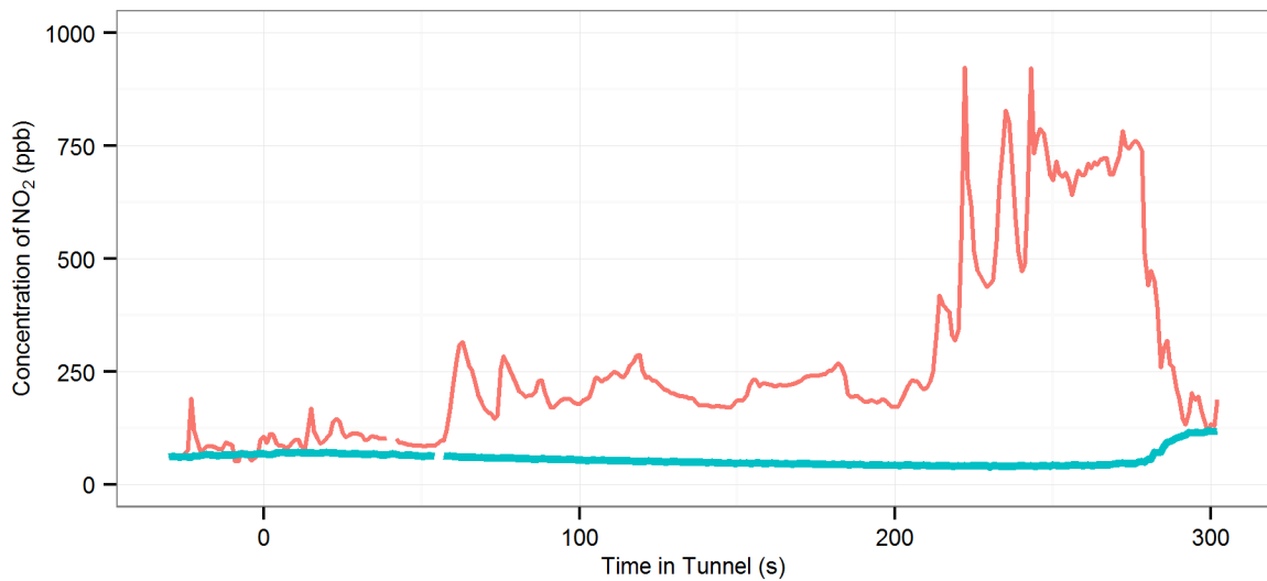
(78) MD2 (R-On | AC-Off | Fn-50%) - Eastern Distributor : Southbound, 2007 Subaru Outback
