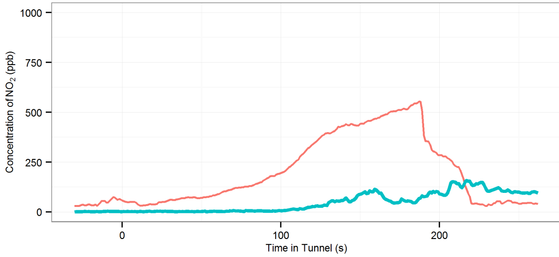
(149) MD5 (R-Off |AC-Off | Fn-0%) - Lane Cove : Eastbound, 2008 Holden Astra Wagon
