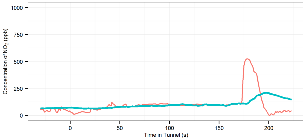
(106) MD4 (R-Off | AC-Off | Fn-50%) - Lane Cove : Westbound, 2002 Ford Fiesta
