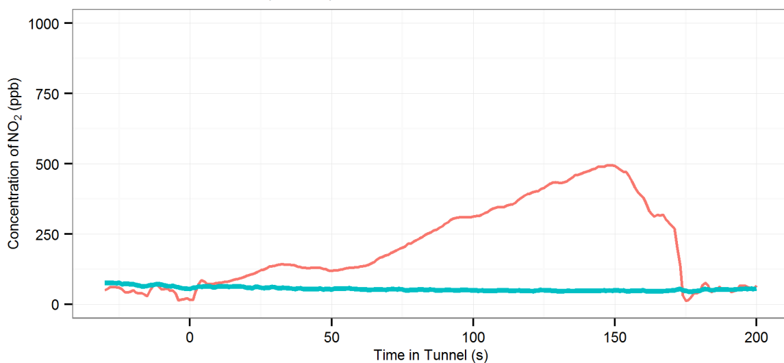
(183) MD3 (R-OnOff | AC-Off | Fn-50%) - Lane Cove : Eastbound, 2008 Toyota Corolla
