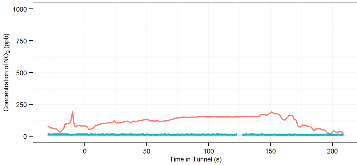
(20) MD2 (R-On | AC-Off | Fn-50%) - Eastern Distributor : Northbound, 2014 Hyundai i30
