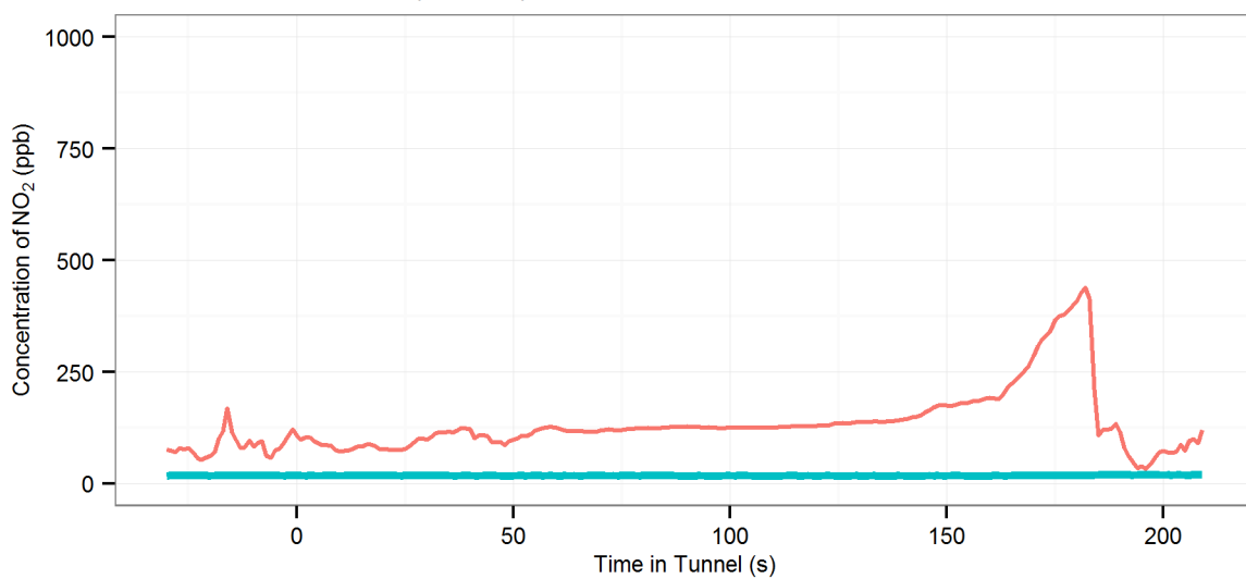
(111) MD2 (R-On | AC-Off | Fn-50%) - Lane Cove : Westbound, 2014 Hyundai i30
