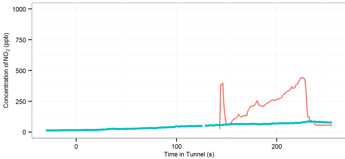
(207) MD4 (R-Off | AC-Off | Fn-50%) - M5E : Eastbound, 2014 BMW X3
