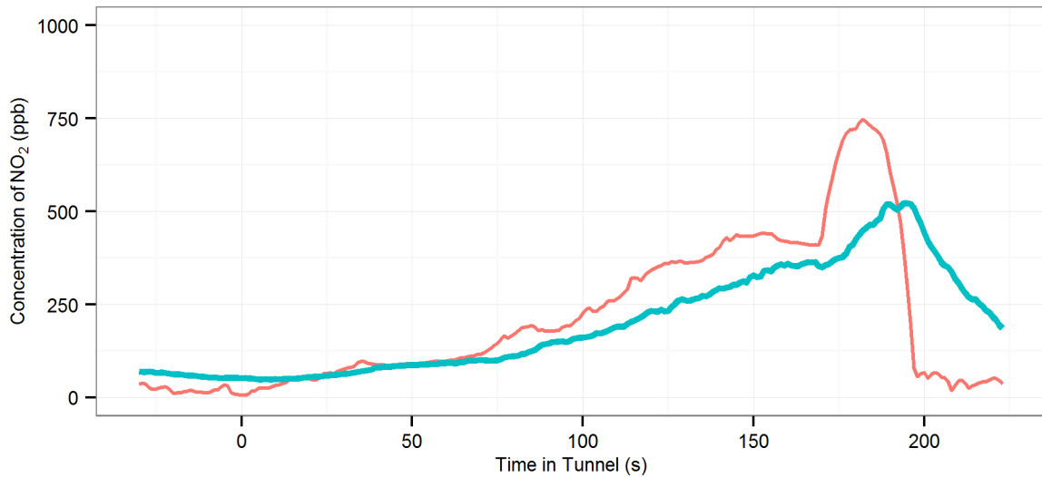
(150) MD6 (R_Off |AC-Off | Fn-100%) - Lane Cove : Eastbound, 2002 Ford Fiesta
