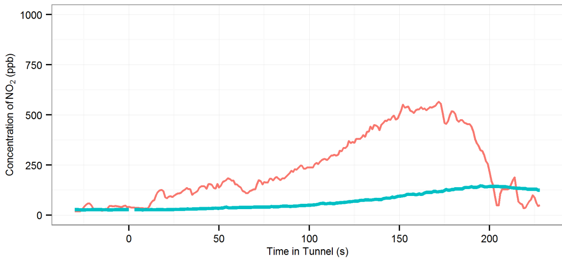
(159) MD6 (R_Off |AC-Off | Fn-100%) - Lane Cove : Eastbound, 2014 BMW X3
