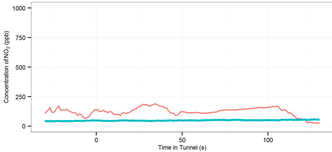
(28) MD4 (R-Off | AC-Off | Fn-50%) - Eastern Distributor : Northbound, 2002 Audi A3
