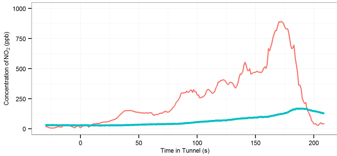
(167) MD3 (R-OnOff | AC-Off | Fn-50%) - Lane Cove : Eastbound, 2002 Audi A3
