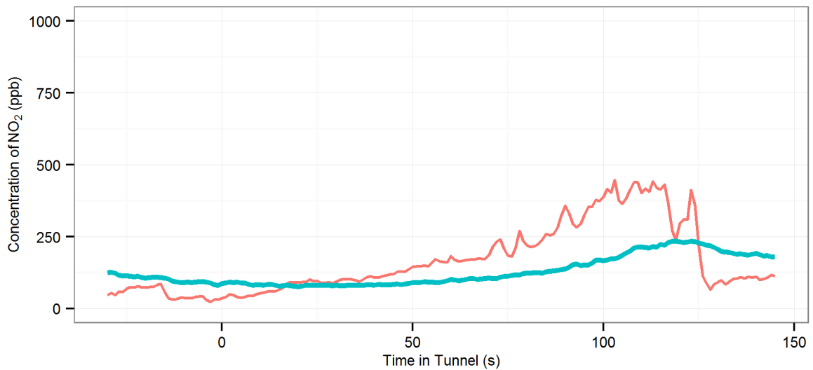
(66) MD4 (R_Off | AC-Off | Fn-50%) - Eastern Distributor : Southbound, 2014 Hyundai i30
