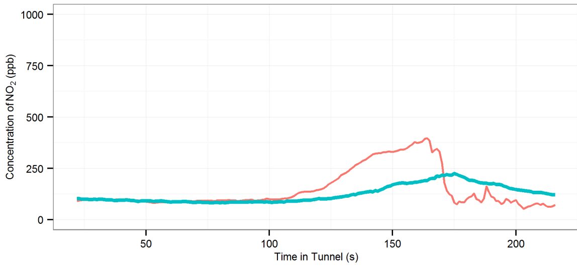
(318) MD4 (R-Off | AC-Off | Fn-50%) - Sydney Harbour : Northbound, 2007 Subaru Outback
