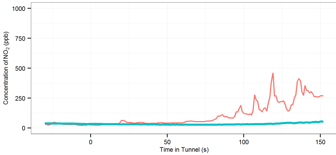
(345) MD6 (R_Off |AC-Off | Fn-100%) - Sydney Harbour : Southbound, 2014 BMW X3
