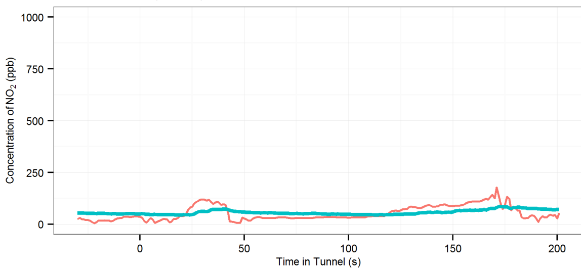
(284) MD4 (R-Off | AC-Off | Fn-50%) - Sydney Harbour : Northbound, 2008 Holden Astra Wagon
