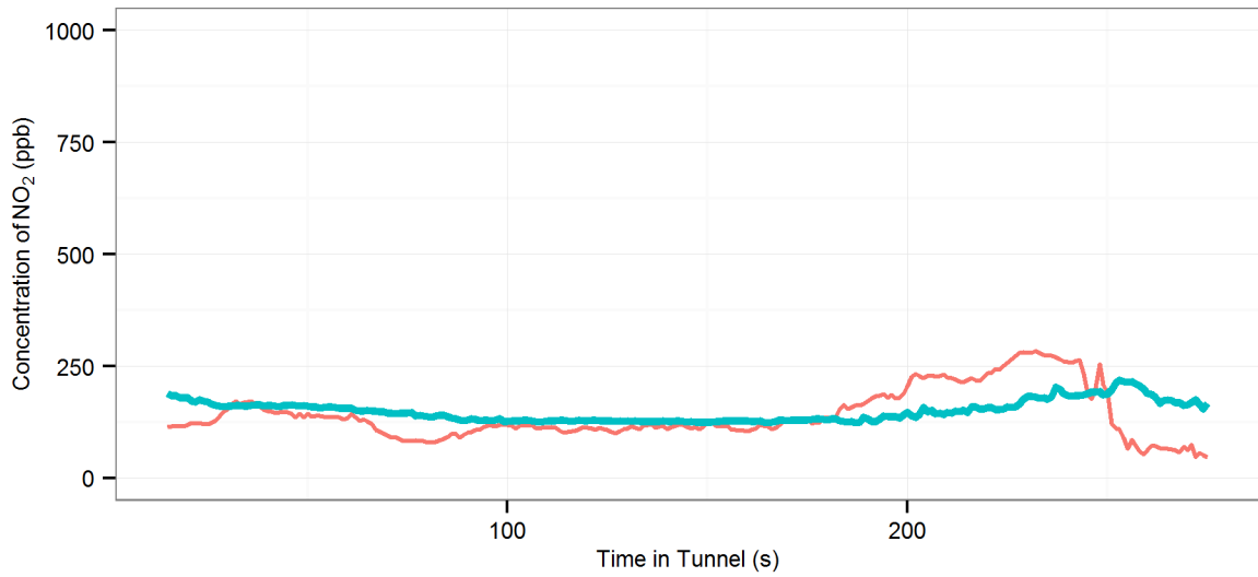
(295) MD4 (R-Off |AC-Off | Fn-50%) - Sydney Harbour : Northbound, 2002 Ford Fiesta
