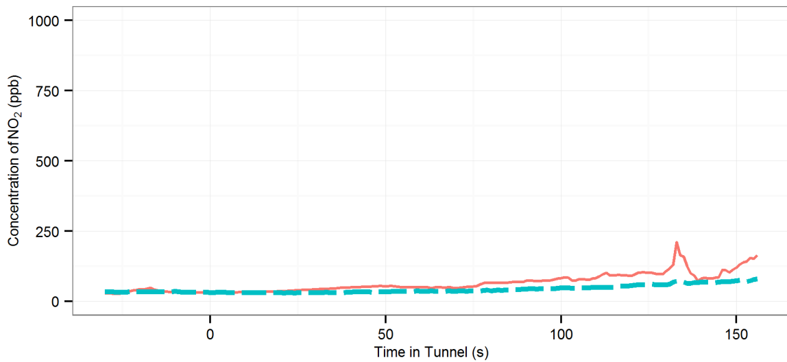
(347) MD6 (R_Off |AC-Off | Fn-100%) - Sydney Harbour : Southbound, 2014 BMW X3
